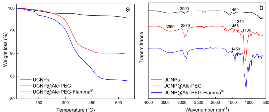
Fig. 3 (a) TGA thermograms and (b) FTIR spectra of UCNPs, UCNPs@Ale-PEG and UCNPs@Ale-PEG-Flamma® particles.
