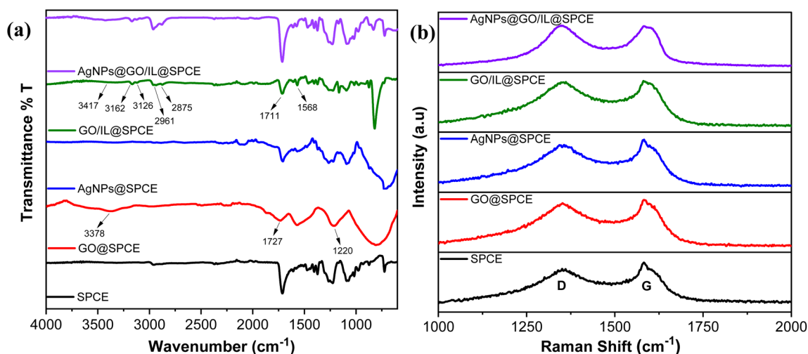
Fig. 3 (a) FT-IR; (b) Raman spectra of SPCE, GO@SPCE, AgNPs@SPCE, GO/IL@SPCE, and AgNPs@GO/IL@SPCE.
