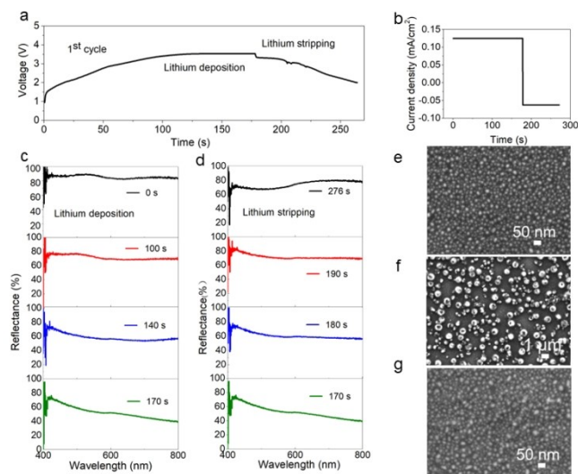
Figure 3 In-situ reflectance and SEM characterization of disorder Li structure during the first cycling. (a) Battery voltage curve of the first cycle. (b) The battery current density profile in the first charging and discharging process. (c) In situ reflectance spectrum during lithium deposition. (d) In situ reflectance spectrum during lithium stripping. (e-g) SEM images of the absorber at stages of the (e) original, (f) Li particles generation and (g) Li stripping states during the first cycle.
