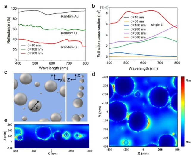
Figure 2 Simulated reflectance and electric field distribution of the lithium nanoparticles. (a) Simulated reflectance of random Au and Li particles. (b) the Simulated extinction cross-section of a single Li particle with different d (diameter). (c) The schematic diagram of random lithium particles, and (d) the simulated electric field distribution of the XY plane at \lambda=605 nm, and (e) the simulated electric field distribution of the XZ plane at \lambda=605 nm.
