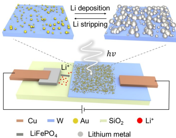
Figure 1 The schematic of the dynamic broadband plasmonic absorber via selective lithium deposition and stripping in a electrochemical lithium metal battery.
