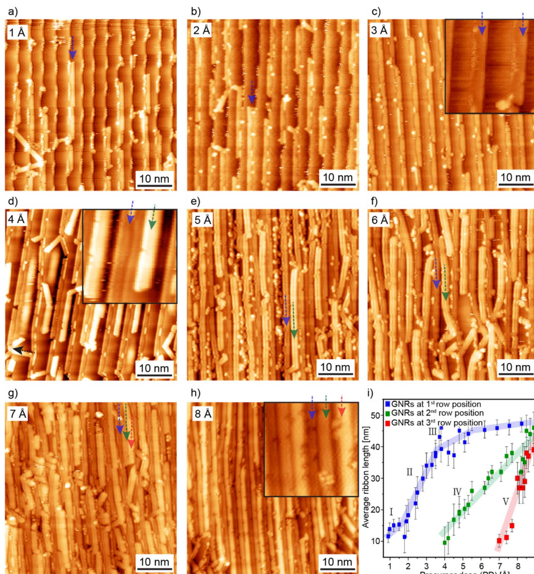
Fig. 1 Evolution of 9-AGNR growth on Au(788) with increasing precursor dose (PD). (a–c) STM images with GNR length evolution at the 1st-row position (blue arrows) along the lower step edges as PD increases from 1 to 3 Å. (d) STM image of GNRs at the 2nd-row position (green arrow) growing parallel to 1st-row GNRs (blue) at PD = 4 Å. (e–f) STM images revealing the length evolution of GNRs at the 2nd-row position (green arrows) at PD = 5 Å and PD = 6 Å, respectively. (g) STM image at PD = 7 Å, revealing the formation of a GNR at the 3rd-row position (red arrow), growing parallel to the GNRs grown previously at the 1st- and 2nd-row positions. (h) STM image of a monolayer of 9-AGNRs with GNRs grown in three parallel rows (blue, green, and red arrows) along each terrace at PD = 8 Å. (i) Histogram illustrating GNR length evolution for 30 samples across all PDs, with error bars representing standard deviation. Tunneling parameters for STM images: V_b = -1.5 V, I_t = 30 pA. Insets in (c), (d) and (h) are zoom-in of the same images for better visualization.
