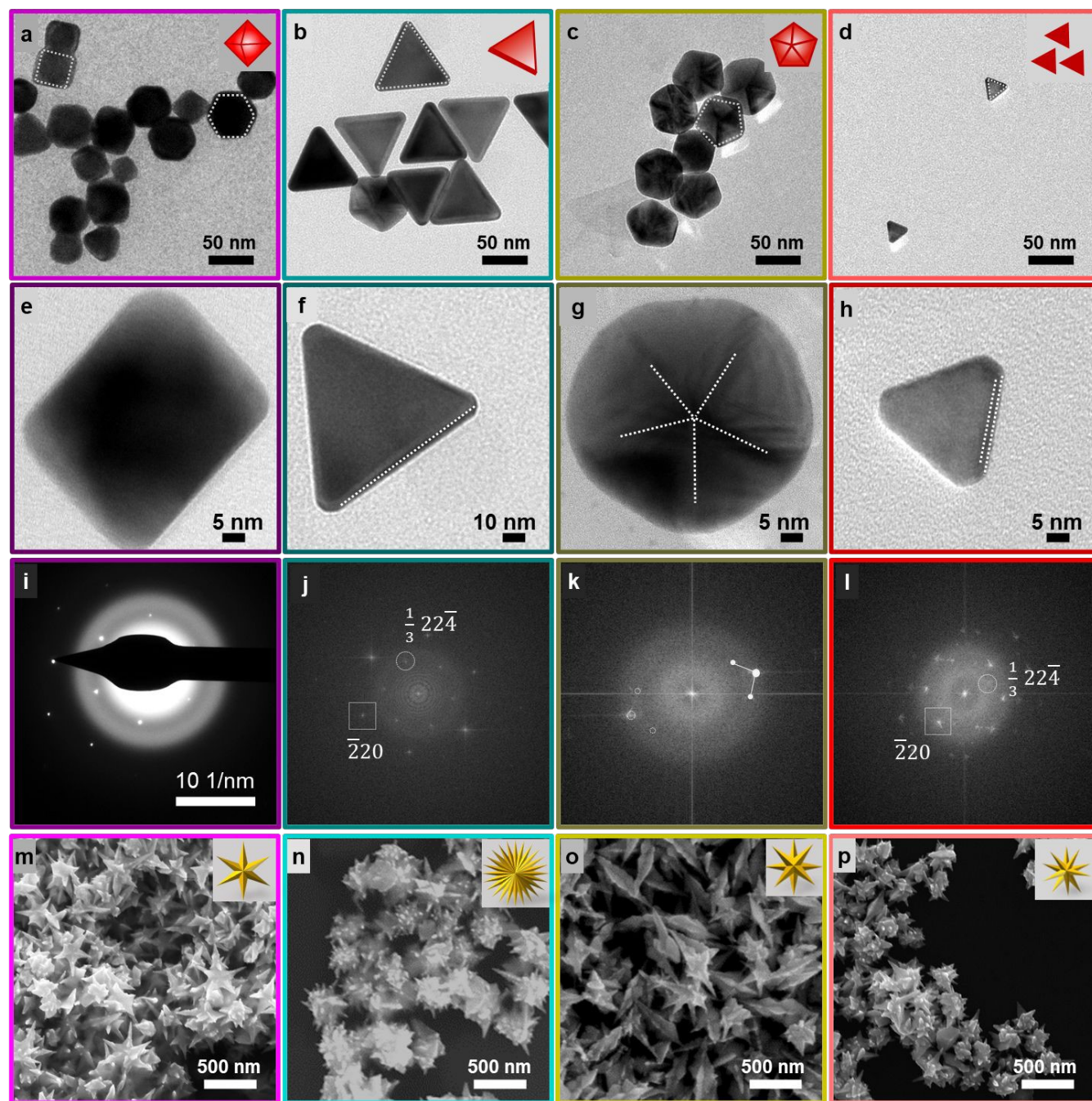
Figure 1. Low magnification TEM images of the different Au NCs used as seeds indicate their successful syntheses and shape purity (a-d) Au octahedra, Au TBT, Au decahedra, and triangular plates, respectively. (e-h) zoomed-in TEM images of four different seeds with distinct defect structure: single crystalline Au octahedra, singly twinned Au TBT NCs, pentatwinned Au decahedra, and triangular plates with stacking faults, respectively. (i-l) Corresponding electron diffraction obtained from Au octahedra and FFT patterns obtained from Au TBT, Au decahedra, and Au triangular plates. (m-p) SEM images of stellated Au NCs overgrown from respective seeds under identical synthetic conditions.
