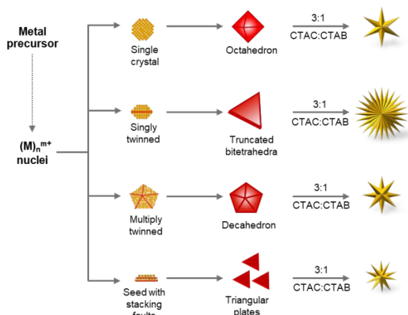
Scheme 1. Schematic representation of the growth of our synthesized Au seeds with different defect structure and morphology but the same {111} surface crystal facets. These Au NCs were subjected to overgrowth under identical synthetic conditions giving rise to stellated Au NCs.
