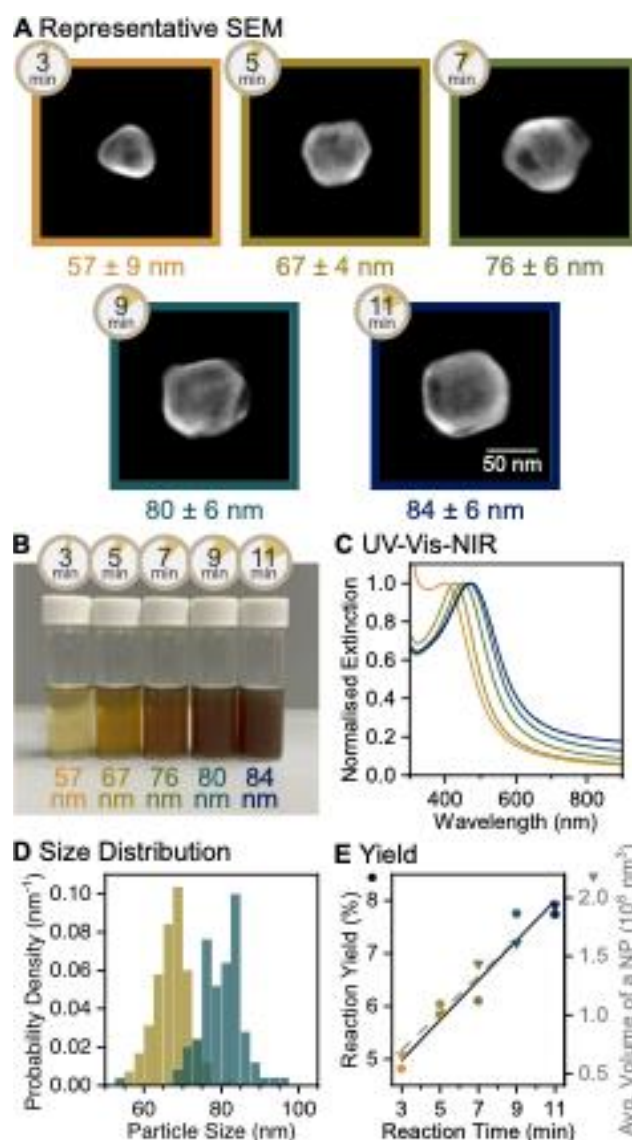
Figure 2. Reaction evolution of the first reduction stage of the growth of faceted Mg NPs, sampled between 3 and 11 min of reaction time. (A) SEM images of representative NPs, labelled with the reaction time as well as average diameter and its standard deviation. (B) Colloidal Mg NPs and (C) their UV-Vis-NIR extinction spectra. (D) Size distribution histogram showing the diameter of Mg NPs obtained from SEM images after 5 and 9 min of reaction, N = 166 and 100 , respectively. Equivalent data for other reaction times are reported in Figure S1. (E) Reaction yield from ICP-OES (circles, black solid line) and average NP volume from SEM images (triangles, grey dashed line) as a function of reaction time showing NP growth; lines represent the linear best fit.
