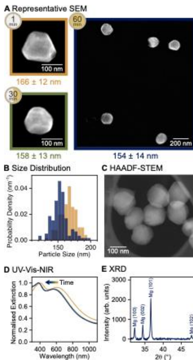
Figure 4. Reaction evolution and outcome of the etching stage in quasi-spherical Mg NP synthesis, sampled between 1 and 60 min of reaction time within this stage, following 5 and 60 min reaction times in first and second reduction stages, respectively. (A) SEM images of representative NPs, labelled with the reaction time as well as average diameter and its standard deviation. (B) Size distribution showing the diameter of Mg NPs obtained from SEM images after 1 and 60 min of reaction, N = 101 and 119 , respectively. Equivalent data after 30 min of reaction are reported in Figure S12. (C) High-angle annular dark-field scanning TEM (HAADF-STEM) image of quasi-spherical Mg NPs. (D) UV-Vis-NIR extinction spectra after 1, 30, and 60 min of reaction. (E) XRD pattern of quasi-spherical Mg
