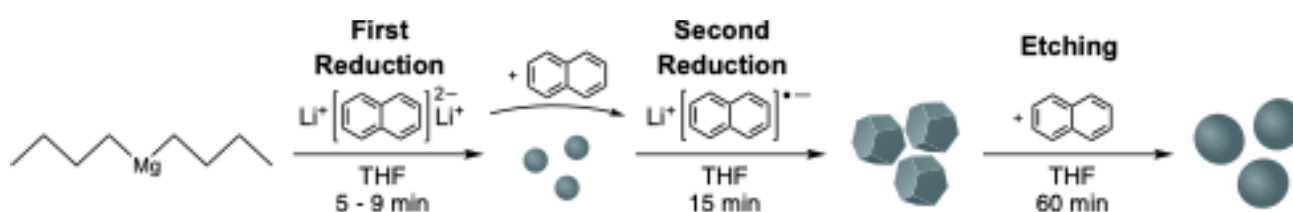
Figure 1. Reaction schematic for the colloidal synthesis of quasi-spherical Mg NPs.
