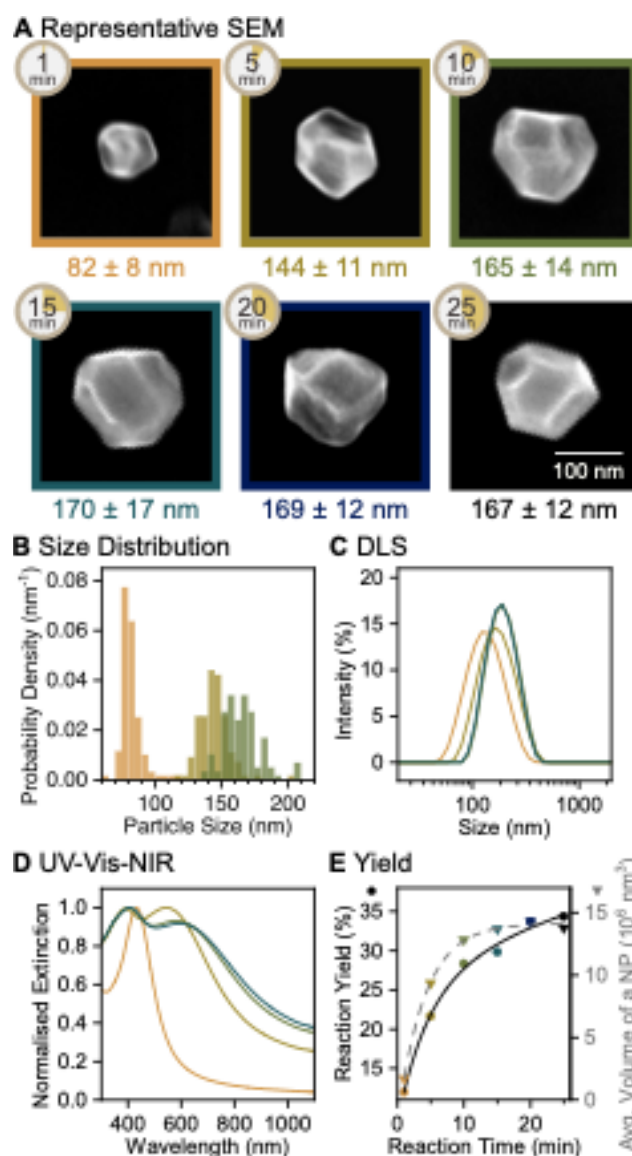
Figure 3. Reaction evolution of the second reduction stage of the growth of faceted Mg NPs, sampled between 1 and 25 min of reaction time within this stage, following a 5 min reaction in the first reduction stage. (A) SEM images of representative NPs, labelled with the reaction time as well as average diameter and its standard deviation. (B) Size distribution histogram showing the diameter of Mg NPs obtained from SEM images after 1, 5, and 10 min of reaction, N = 119 , 109, and 117, respectively. Equivalent data for other reaction times are reported in Figure S7. (C) Size distribution of Mg NPs after 1, 5, 10, and 15 min of reaction obtained from DLS and (D) their UV-Vis-NIR extinction spectra. Equivalent data for other reactions are reported in Figures S8 and S9. (E) Reaction yield from ICP-OES (circles, black
