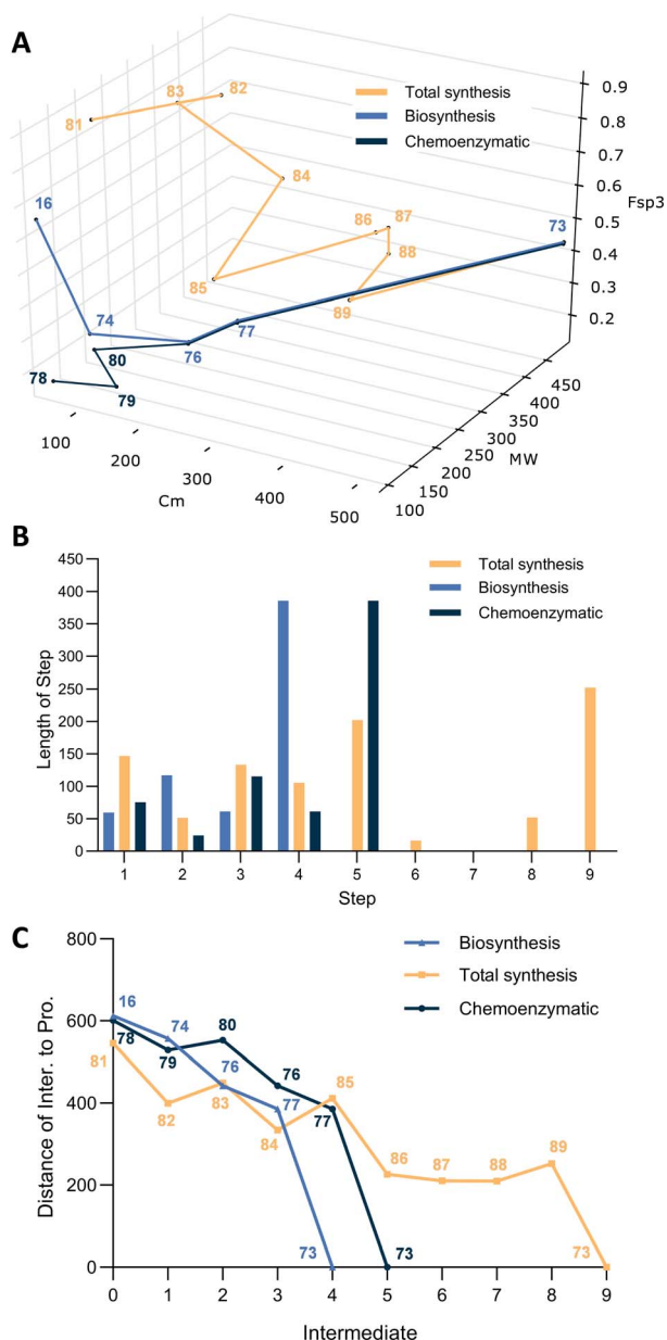
Fig. 5 Chemical space analysis for the production of bisorbicillinol 73 . (A) The biosynthesis and chemical synthesis of bisorbicillinol 73 illustrated as a C_{mw} , MW and F_{sp3} parameterized 3D plot; (B) bar chart of distance for each step; (C) line chart of distances of each intermediate to final product.
