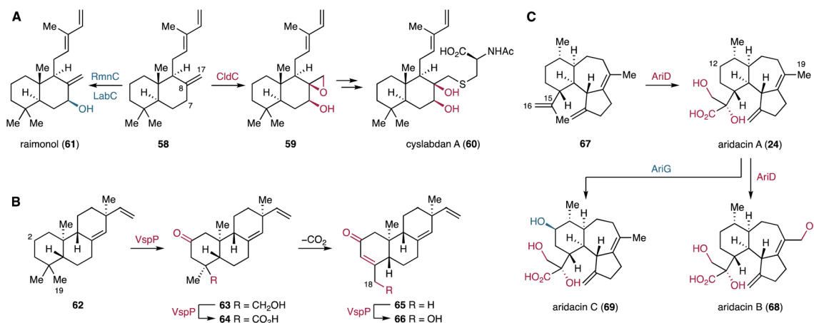
Fig. 11 Representative examples of bacteria terpenoid functionalization by multifunctional P450s. Proposed biosynthesis of cyclabdan A and raimonol (A), ent -sandarapimaradiene derived diterpenoids (B), and aridacins (C).
