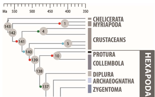
Fig. 1 Phylogenetic relationship of Collembola with other arthropods, adopted from Misof et al. Science , 2014, 346 , 763. 3 Collembola are basal hexapods. Recent insect lineages evolved mostly much later. The arthropods went ashore about 400 mya, with the three lineages Chelicerata, Myriapoda, and Hexapoda, while Crustacea mostly stayed in water. Reprinted with permission from AAAS.
