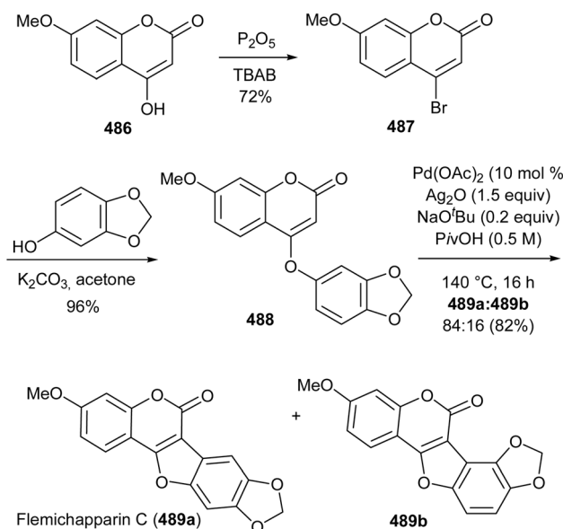
Scheme 70 Synthesis of flemichapparin C (489a).
