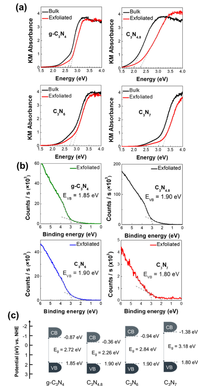
Fig. 5 (a) UV-Vis absorption spectra, (b) UPS spectra, and (c) schematic illustration of the band position for exfoliated g-C_3N_4 , C_3N_{4.8} , C_3N_6 , and C_3N_7 nanosheets.
