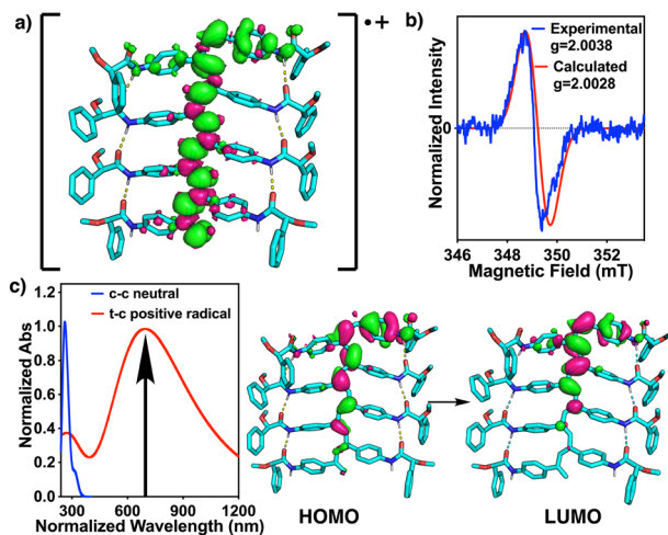
Fig. 5 (a) Spin density of a radical cation oligomer with a trans-cisoidal structure. (b) Comparison between the experimental EPR of poly-( R )-1/ M^{n+} and that calculated for the trans-cisoidal oligomer. (c) Simulated UV-Vis spectra of the neutral cis-cisoidal oligomer and the radical cation trans-cisoidal oligomer. Transition attributed to the band at ca. 700 nm in the radical cation trans-cisoidal oligomer.
