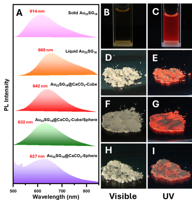
Fig. 3 (A) PL intensity of solid \text{Au}_{22}\text{SG}_{18} , liquid \text{Au}_{22}\text{SG}_{18} , \text{Au}_{22}\text{SG}_{18}@CaCO_3 -Cube, \text{Au}_{22}\text{SG}_{18}@CaCO_3 -Cube/Sphere, \text{Au}_{22}\text{SG}_{18}@CaCO_3 -Sphere and. Digital images of (B and C) liquid \text{Au}_{22}\text{SG}_{18} , (D and E) \text{Au}_{22}\text{SG}_{18}@CaCO_3 -Cube, (F and G) \text{Au}_{22}\text{SG}_{18}@CaCO_3 -Cube/Sphere, (H and I) \text{Au}_{22}\text{SG}_{18}@CaCO_3 -Sphere taken under visible and UV ( \lambda_{ex} = 520 nm).
