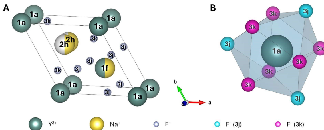
Figure 1. (A) Unit cell of \beta - \text{NaYF}_4 with the composition \text{Na}_{1.5}\text{Y}_{1.5}\text{F}_6 . Dark green spheres represent \text{Y}^{3+} , yellow spheres \text{Na}^+ , white spheres are unoccupied sites, and small grey spheres represent \text{F}^- . Half spheres indicate a 50% occupation. (B) Both possible doping sites for \text{Ln}^{3+} (i.e., 1a and 1f) are coordinated in a tricapped trigonal prismatic geometry by nine \text{F}^- . For clarity, the three 3j (caps) and the six 3k (trigonal prism) \text{F}^- are coloured in cyan and in pink, respectively. The prism for the 1f site is generated by rotating the coordination polyhedron shown in (B) by ca. 90^\circ around the c-axis and swapping of the Wyckoff symbols for all \text{F}^- .
