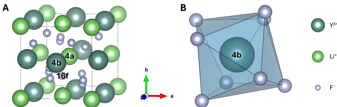
Figure 4. (A) Unit cell of LiYF 4 with the composition Li 4 Y 4 F 16 . Dark green spheres represent Y 3+ , light green spheres Li + , and small grey spheres represent F - . LiYF 4 features only one potential doping site, i.e., Wyckoff position 4b. (B) Coordination polyhedron around Y 3+ . Each Y 3+ at a 4b site is surrounded by eight F - ions, creating a distorted square antiprism.
