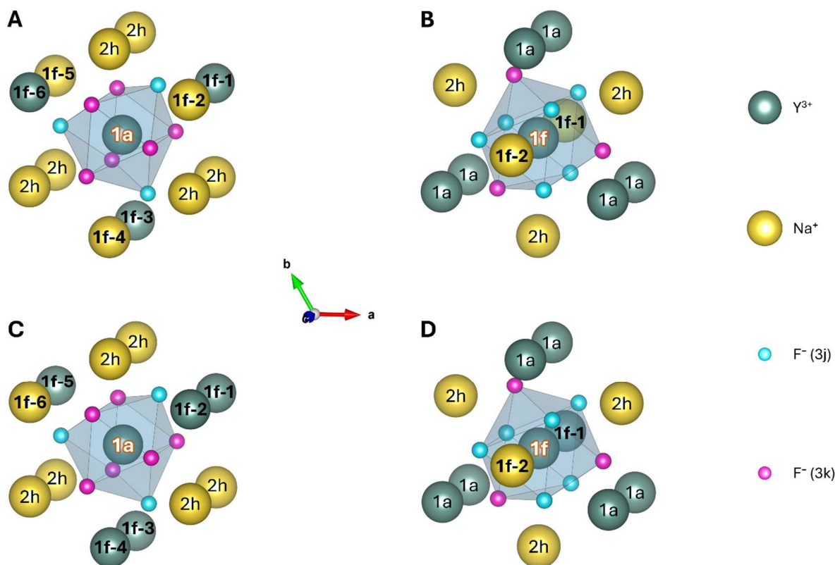
Figure 3. Zoom-in onto the potential (A) 1a and (B) 1f doping sites and their first anionic and cationic coordination spheres for the supercells shown in Figure 2A and B, respectively. The corresponding supercells are designated as configuration (A) 10 and (B) 1 in Table 1. Zoom-ins of two additional configurations are shown in C and D, corresponding to configuration 15 and 2, respectively, in Table 1. Here some of the 1f sites were altered in comparison to configuration 10 and 1. For all clusters the 1a, 1f, and 2h sites are labelled by their Wyckoff symbols, the central site is labelled in white. The 1f sites for which the distribution of Na + and Y 3+ were altered in this study are set in bold and numbered from (1f-) 1 to 6 (panels A and C) and 1 to 2 (panels B and D) for the potential 1a and 1f doping sites, respectively. The numbering of these sites is equivalent to the scheme used in the last column of Table 1. All clusters presented here were created for visualisation purposes only and are still embedded in their respective supercells used for the geometry optimisation.
