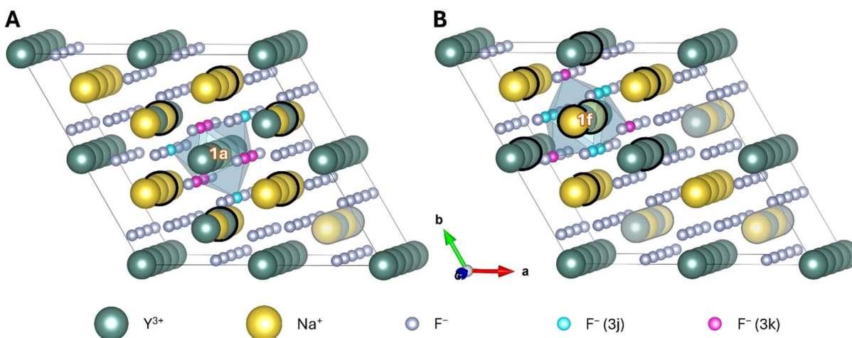
Figure 2. 2x2x4 supercell of \beta -NaYF 4 with the composition Na 24 Y 24 F 96 . Highlighted are a potential (A) 1a and (B) 1f doping site (white labels), and their first anionic (F - ions of the blue prism that are highlighted in cyan and pink) and cationic (Na + and Y 3+ ions marked with a thick black line) coordination spheres. Na + and Y 3+ at the not neighbouring 1f rows (represented as faint) were not exchanged when creating the different configurations of the supercell. All other 1f sites were altered successively. For better visualisation of the two potential doping sites and their closest ions, a close-up of the two potential doping sites with their nearest ions is shown in Figure 3A and B.
