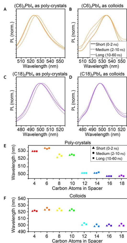
Figure 4 – TRPL of 2D (C_n)_2PbI_4 MHP in 3 time frames of the PL decay – 0–2 ns, 2–10 ns, and 10–60 ns. A. (C_6)_2PbI_4 as poly-crystals, and B. as colloids. C. (C_{18})_2PbI_4 as poly-crystals, and D. as colloids. E. Comparison of the PL peaks wavelength at the different time frames of poly-crystals and, F. of colloids.
