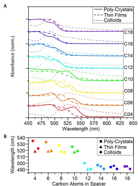
Figure 2 – Absorbance of 2D (C n ) 2 PbI 4 MHP. A. Absorbance spectra of C4-C18, as poly-crystals, thin-films and colloids B. Comparison of exciton wavelengths.
