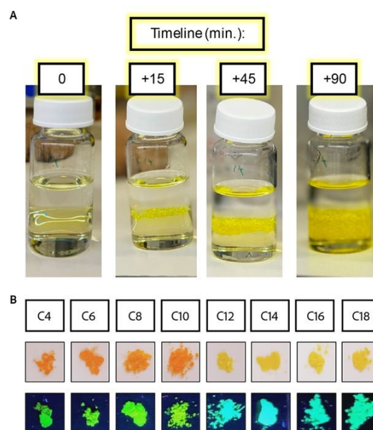
Figure 1 – A. Photos taken during the synthesis of poly-crystals with long ligands ( C \geq 12 ), growing in the interphase between methanol and HI. B. Photos of the obtained poly-crystals under white light, and under UV light (bottom).
