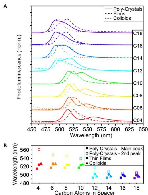
Figure 3 – Steady-state PL of 2D (C_n)_2PbI_4 MHP. A. PL spectra of C4-C18, as poly-crystals, thin-films and colloids. B. Comparison of the PL peaks wavelengths.
