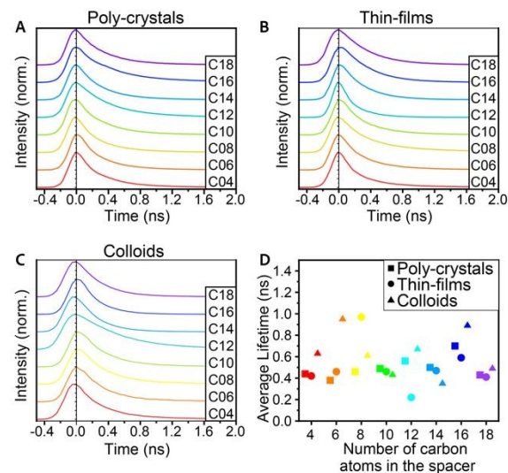
Figure 5 – PL decay spectra of 2D (C_n)_2PbI_4 MHP, for A. poly-crystals, B. thin-films, and C. colloids. D. Averaged lifetime of PL decay for poly-crystals, thin-films, and colloids.
