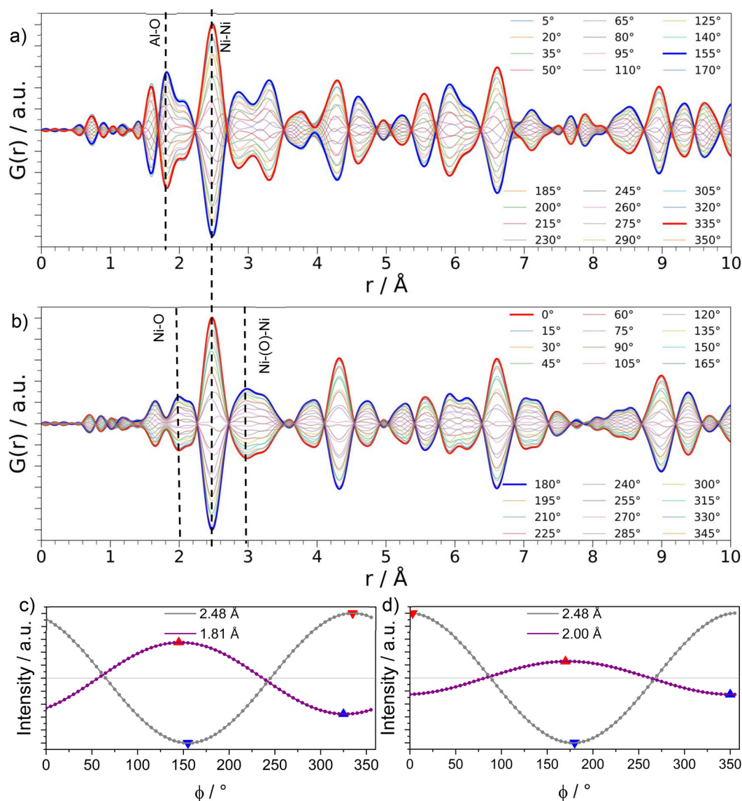
Fig. 2 PSD-transformed data for Ni@SbA150 (a) and SPP2080-IMRC (b). The data are shown for values of the phase \phi from 0^\circ to 360^\circ with an angular resolution of 15^\circ . The in-phase angle is shown in red ( 335^\circ for Ni@SbA150 and 0^\circ for SPP2080-IMRC), while the anti-phase angle is shown in blue ( 155^\circ for Ni@SbA150 and 180^\circ for SPP2080-IMRC). For Ni@SbA150, in (c), the variation of intensity for the peaks at 2.48 \text{ \AA} (Ni–Ni distance in the \text{Ni}_{\text{fcc}} structure) and 1.81 \text{ \AA} (Al–O distance in the \gamma\text{-Al}_2\text{O}_3 structure) is shown as a function of the PSD angle \phi . For SPP2080-IMRC, in (d), the variation of intensity is shown for the peaks at 2.48 and 2.00 \text{ \AA} , with the latter being attributed to the Ni–O distance in the NiO structure. The red triangles represent the in-phase angles and the blue triangles the anti-phase angles.
