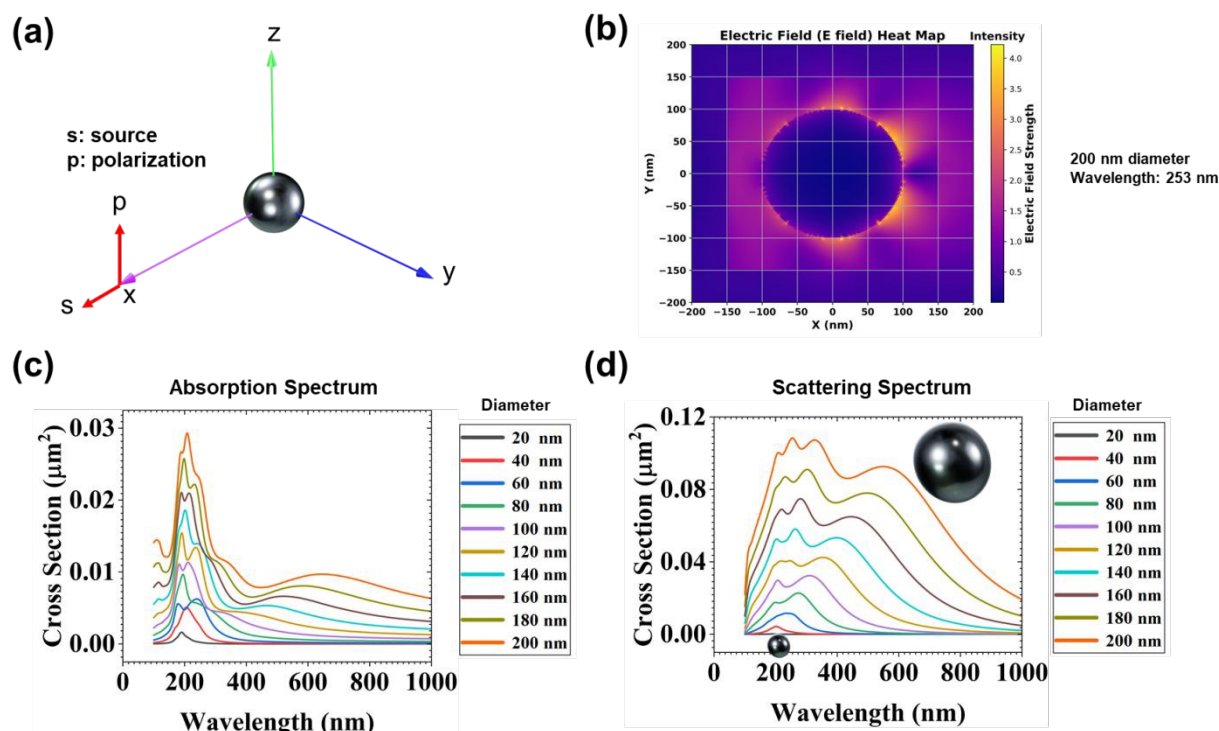
Figure 1. Plasmonic resonance behavior of a single spherical EGaIn nanoparticle. (a) 3D schematic of a single spherical EGaIn NP excited by a plane-wave light source (s) with 90° polarized angle (p). (b) Electrical field (E field) heat map for a 200-nm diameter spherical EGaIn nanoparticle excited at 253-nm wavelength (corresponding to its major scattering peak). The plane-wave light source propagates in x-direction from left to right. (c) Absorption and (d) scattering cross-section spectra of single spherical EGaIn nanoparticles with various diameters (20-200 nm).
