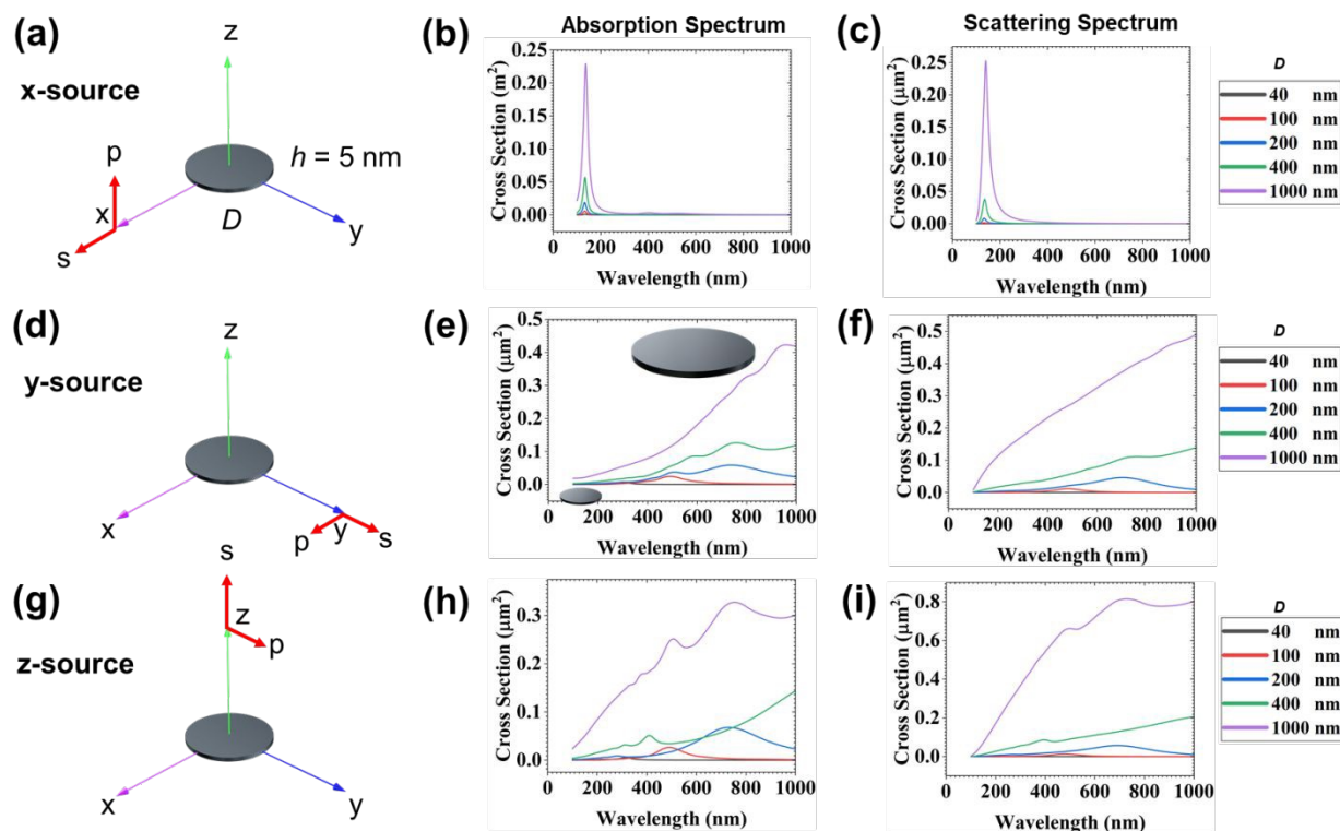
Figure 5. Plasmonic resonance behavior of single EGaIn nanodisk. (a), (d), and (g) 3D schematic of single EGaIn nanodisk excited by a plane-wave light source (s) in x-, y-, and z-directions with 90 degree polarization (p), respectively. (b), (e), and (h) Absorption and (c), (f), and (i) scattering cross-section spectrums for various diameters with fixed 5 nm thickness.
