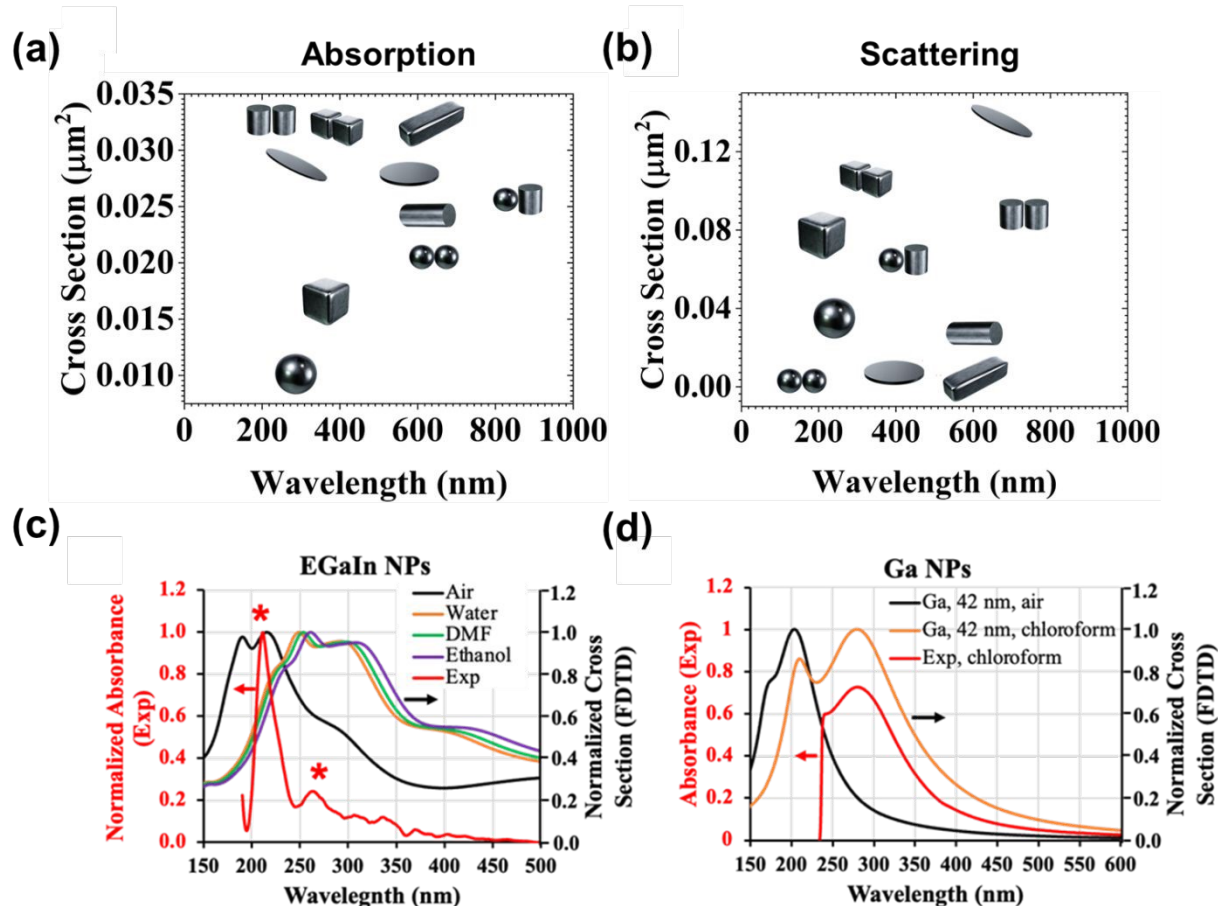
Figure 7. Map of EGaIn nanoplasmonics and experimental validation. Peak absorption (a) and scattering (b) wavelengths and corresponding cross-sections for different shapes that have been simulated by FDTD. (c) Overlap of experimental UV-vis absorption spectrum of EGaIn nanoparticles (185 nm by DLS) in ethanol with FDTD simulated absorption cross-section (160 nm) in different media (air, water, DMF, and ethanol). Red asterisks denote the major UV absorption peaks of synthesized EGaIn nanoparticles. (d) Overlap of experimental UV-vis absorption spectrum of Ga nanoparticles (42 nm by TEM) in chloroform with FDTD simulated absorption cross-section (42 nm) in different media (air and chloroform). The experimental UV-vis spectrum shows the UV cutoff effect of chloroform for wavelength shorter than ~245 nm.
