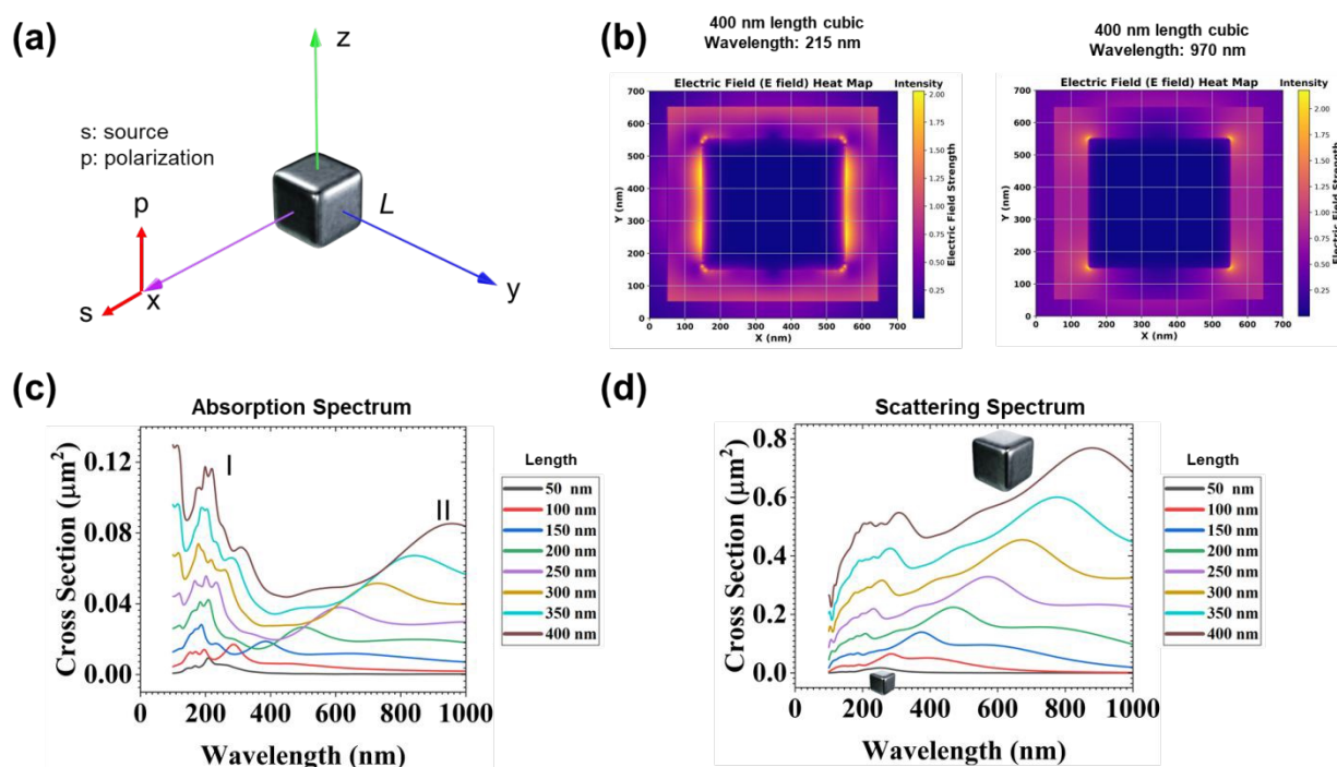
Figure 2. Plasmonic resonance behavior of single cubic EGaIn nanoparticle. (a) 3D schematic of single cubic EGaIn nanoparticle excited by a plane-wave light source (s) in x-direction with a 90 degree polarization (p) angle. (b) Electrical field (E field) heat map for a 400-nm length cubic EGaIn nanoparticle excited at 215 nm and 970 nm wavelength (major absorption peaks), respectively. The plane-wave light source propagates in x-direction from left to right. (c)
