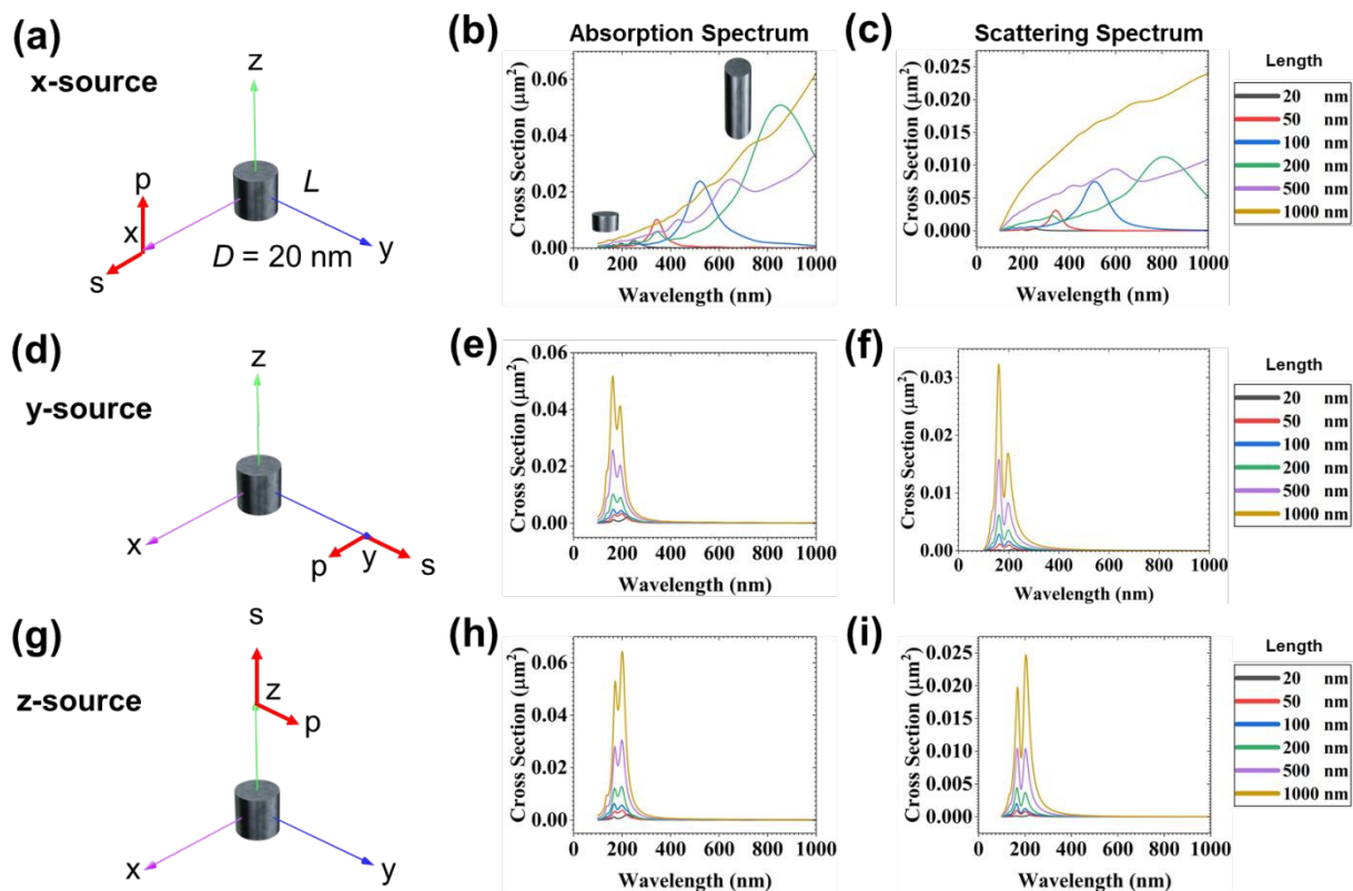
Figure 3. Plasmonic resonance behavior of single EGaIn nanorod. (a), (d), and (g) 3D schematic of single EGaIn nanorod excited by a plane-wave light source (s) in x-, y-, and z-directions with 90 degree polarization (p), respectively. (b), (e), and (h) Absorption and (c), (f), and (i) scattering cross-section spectra for various lengths with a constant diameter of 20 nm.
