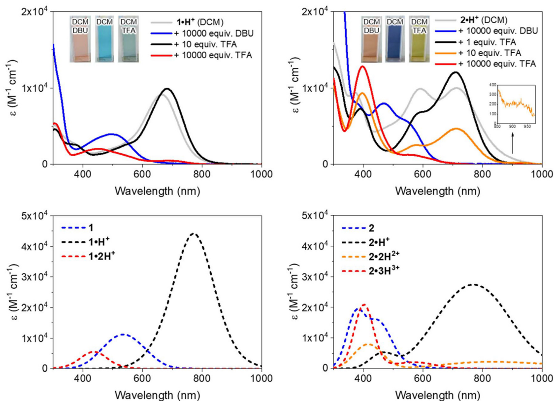
Fig. 4 Top: electronic absorption spectra of 1 \cdot \text{H}^+ (left) and 2 \cdot \text{H}^+ (right) in DCM (ca. 10^{-5} M) without or with the presence of DBU (1,8-diazabicyclo (5.4.0)undec-7-ene) or TFA (trifluoroacetic acid). Bottom: theoretically determined electronic absorption spectra of the protonation states of 1 (left) and 2 (right) in DCM.
