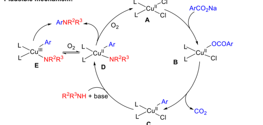
Scheme 4 Cu-catalyzed decarboxylation of aromatic carboxylic acids.
