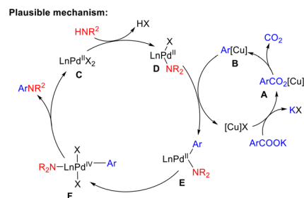
Scheme 11 Mechanism of Pd/Cu co-catalyzed decarboxylative amination.
