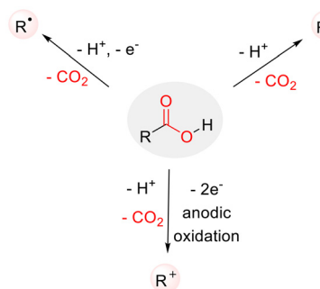
Scheme 2 Three possible mechanisms for the decarboxylative process of carboxylic acids.
