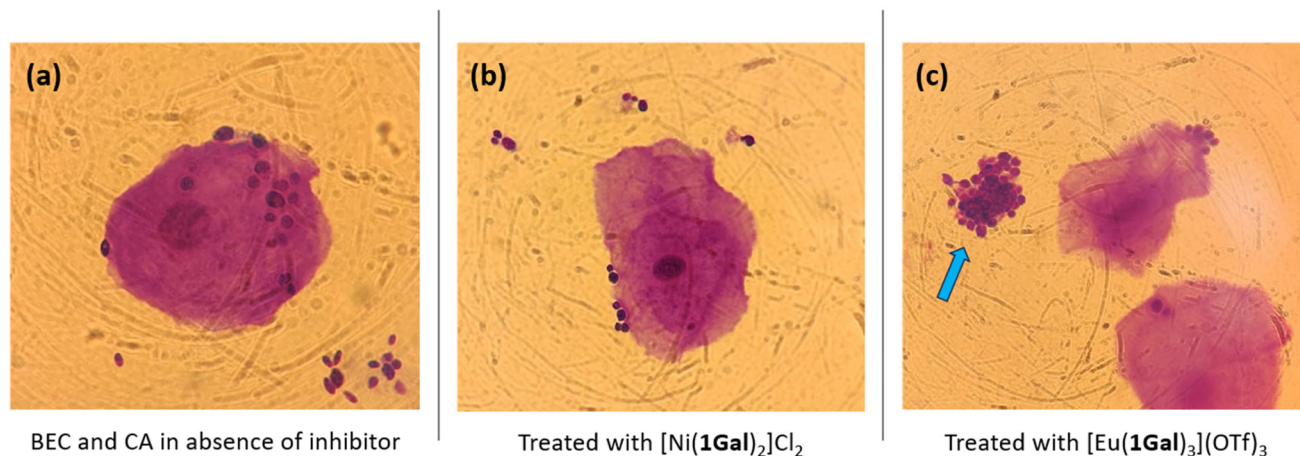
Fig. 7 Optical microscope images (100x) of human buccal epithelial cells (BECs) in the presence of C. albicans (a) without any inhibitor (control sample); (b) in competition assay with the Ni(II) complex, demonstrating smaller fungal cells; (c) in competition assay with 1:3 Eu(III) complex, demonstrating clumping of C. albicans cells (indicated with arrow) and human BECs with minimal fungal adhesion.
