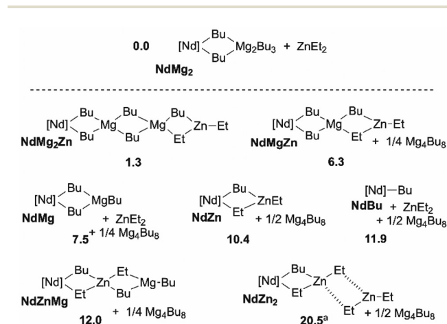
Scheme 3 Speciation of the alkylated species yielded from [\text{Nd}]-^n\text{Bu} , \text{Mg}_4^{\text{n}}\text{Bu}_8 and \text{ZnEt}_2 . Only the most stable species are shown, the fully detailed speciation is provided in ESI.† ΔG in kcal mol -1 . a In NdZn 2 , interaction between the \text{ZnEt}_2 fragments is weak, the endergonicity results from the entropy cost of the association of free and separated \text{ZnEt}_2 . Gaussian 09, B3PW91/D3BJ(SP), SMD(TolH), 298 K, 1 atm.
