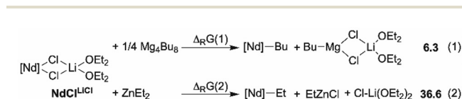
Scheme 2 Thermodynamics ( \Delta_R G , kcal mol −1 ) of [\text{Nd}]\text{-R} species formation ( \text{R} = \text{}^n\text{Bu} or \text{Et} ) as a function of the alkylating agent. [\text{Nd}] corresponds to the metal center and its \text{Me}_2\text{Si}(\text{C}_{13}\text{H}_8)_2 ligand. Gaussian 09, B3PW91/D3BJ(SP), SMD(TolH), 298 K, 1 atm.
