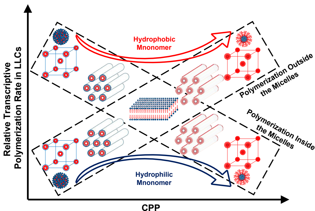
Fig. 8: Proposed relationship between CPP of the structure and transcriptional polymerization rate
