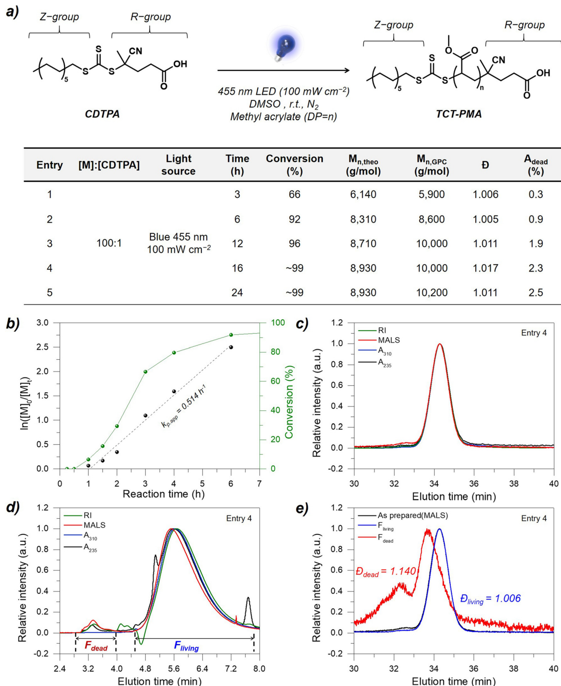
Fig. 2 (a) Scheme of photoiniferter-RAFT polymerization of poly(methyl acrylate) using CDTPA as an iniferter in DMSO under a blue LED ( \lambda_{max} = 455\text{ nm} , 100\text{ mW cm}^{-2} ). A_{dead} (%) = area of fraction/(area of all polymer peaks) \times 100 . (b) Pseudo-first order kinetic plot (black) and respective monomer conversion plot (green). (c) GPC chromatogram of as-prepared PMA at 16 hours of reaction, RI (green): refractive index detector signal, R_{90} (red): multi-angle light scattering detector signal, A_{310} (blue): UV detector signal at 310 nm, and A_{235} (black): UV detector signal at 235 nm. (d) HPLC chromatogram of as-isolated PMA at 16 hours of reaction. (e) GPC chromatograms of fractioned " F_{dead} " and " F_{living} ".
