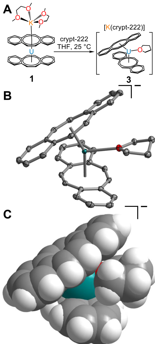
Fig. 4 (A) Synthetic route to [K(crypt-222)][U(dbCOT) 2 (THF)] − , 3 . (B) Structure of the [U(dbCOT) 2 (THF)] − anion in a crystal of [K(crypt-222)][U(dbCOT) 2 (THF)] − , 3 , with thermal ellipsoids drawn at the 50% probability level. Teal, red, and grey ellipsoids represent U, O, and C atoms, respectively. H atoms and the [K(crypt-222)] + counteranion are omitted for clarity. (C) Space filling model of the [U(dbCOT) 2 (THF)] − anion in a crystal of [K(crypt-222)][U(dbCOT) 2 (THF)] − , 3 . Teal, red, grey, and white-grey spheres represent U, O, C, and H atoms, respectively. The [K(crypt-222)] + counteranion is omitted for clarity. Select interatomic distances (Å) and angles (°) for 3 : U–C COT = 2.692(3)–2.939(3); U–Cnt = 2.106, 2.128; Cnt–U–Cnt: 150.4. We define that the circles in each dbCOT drawing represent in total 18 \pi -electrons.
