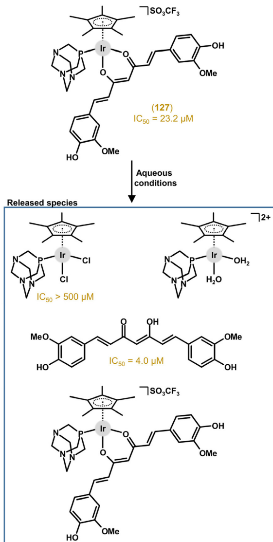
Fig. 50 The structural formula of complex 127 and the route to its decomposition in the presence of water (water : DMSO mixture; ^1\text{H} , ^{31}\text{P} NMR studies), given together with the IC 50 values determined in A2780 cells.
