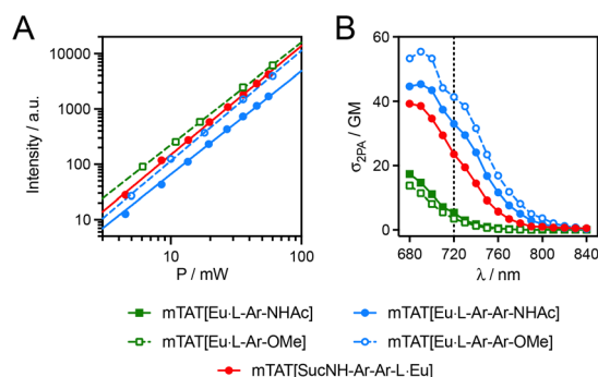
Fig. 5 2P spectroscopy: (A) quadratic power dependence of the \text{Eu}^{3+} emission ( \lambda_{\text{ex}} = 730 nm) for mTAT[Eu-L-Ar-R] ( R = \text{Ar-OMe} , \text{Ar-Ar-NHAc} and \text{Ar-Ar-OMe} ) and mTAT[SucNH-Ar-Ar-L-Eu] in PBS. Data were fitted using I = A \times P^n yielding n = 1.85 , 1.87 , 1.99 and 1.97 , respectively. (B) 2P absorption spectra measured in PBS. The vertical dotted line corresponds to the 2P excitation wavelength used for cell microscopy imaging. Measurements were performed in PBS pH 7.4.
