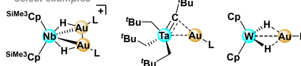
Fig. 1 Established synthetic routes to heterometallic gold coordination complexes. Low-valent mixed-metal gold complexes are generally accessed via salt-metatheses with transition metal polycarbonyls (A). High-valent M/Au compounds are routinely prepared via treatment of hydride or alkyl complexes with appropriate gold(I) precursors (B).
