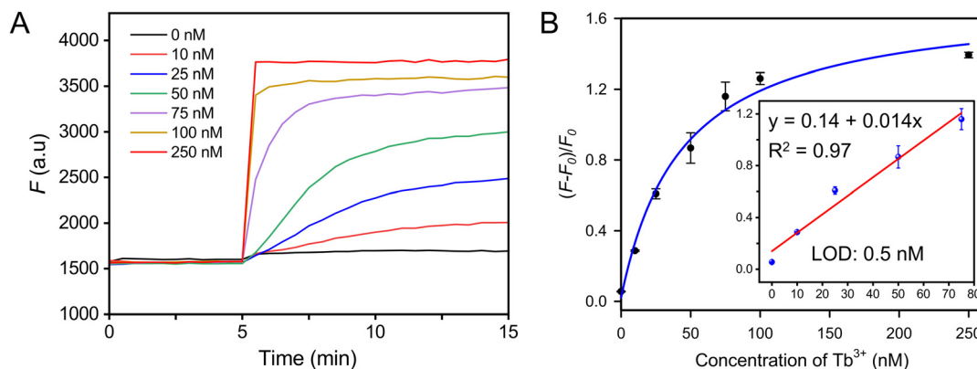
Fig. 5 Fluorescent strand-displacement aptamer biosensor for the detection of Tb^{3+} in Lake Ontario water. (A) Kinetics traces of the 20 nM biosensor in the presence of various concentrations of Tb^{3+} in lake water. (B) The calibration curve of the sensor. Inset: linear response at low Tb^{3+} concentrations. The water contained 10 mM MES, 100 mM NaCl, and 2 mM MgCl_2 , with the pH adjusted to 6.
