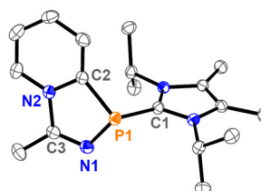
Fig. 1 Molecular structure of 9a 2+ in 9a [OTf] 2 (hydrogen atoms and counter ions are omitted for clarity; thermal ellipsoids are displayed at 50% probability). Selected bond lengths in Å and angles in (°): P1–C1 1.8145(13), P1–N1 1.7122(12), P1–C2 1.8199(14), N1–C3 1.2689(19), C3–N2 1.4606(18), N1–P1–C1 105.27(6), N1–P1–C2 91.72(6), C1–P1–C2 107.50(6), N2–C2–P1–N1 13.20(9).
