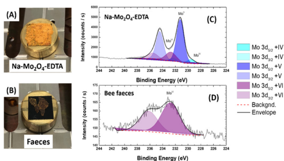
Fig. 8 Samples of Na-Mo 2 O 4 -EDTA and bee faeces deposited on carbon tape (A and B, respectively). The diameter of the sample holder is 1 cm; XPS high-resolution spectra (Mo3d region) of Na-Mo 2 O 4 -EDTA (C) and bee faeces (D). The different contributions and the background used for the reconstruction are plotted as well as the final envelope.
