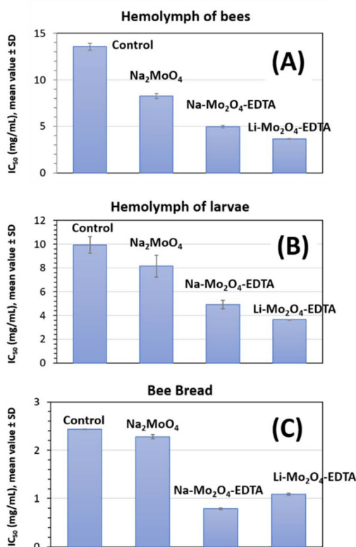
Fig. 9 Antioxidant properties of hemolymph of worker bees (A) and larvae (B) and beebread (C) obtained from beehives of the control group or the groups fed with Na 2 MoO 4 ·2H 2 O, Na-Mo 2 O 4 -EDTA and Li-Mo 2 O 4 -EDTA. Each IC 50 value corresponds to an average value between three replicates.
