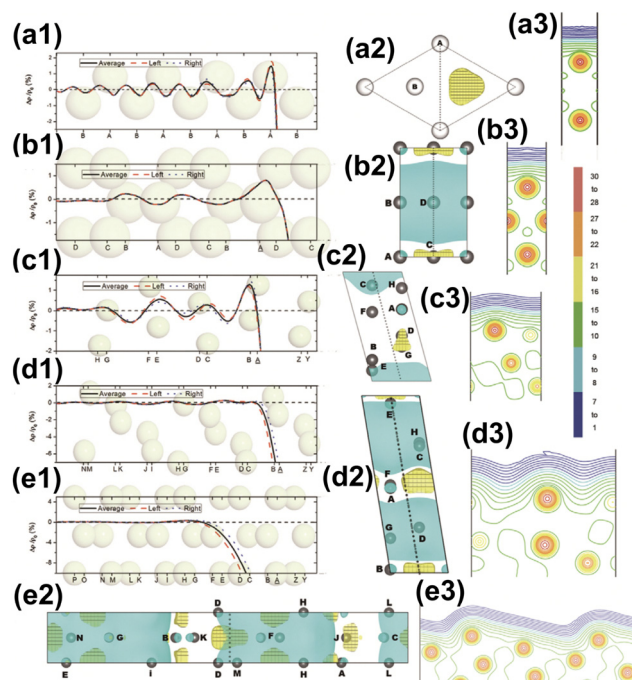
Fig. 30 Friedel oscillations as a function of the depth z are shown for (a1) Mg(0001), (b1) Mg(1010), (c1) Mg(1011), (d1) Mg(1013) and (e1) Mg(1018). Subsequent top-down views of charge transfer are presented for (a2) Mg(0001), (b2) Mg(1010), (c2) Mg(1011), (d2) Mg(1013) and (e2) Mg(1018). Cross-sectional views of charge densities are displayed for (a3) Mg(0001), (b3) Mg(1010), (c3) Mg(1011), (d3) Mg(1013) and (e3) Mg(1018). The topmost surface layer is indicated with an underline. In the charge transfer sections specifically in graphs (a2), (b2), (c2), (d2), and (e2) light blue and yellow squares represent charge depletion and accumulation in the surface region. The color bar illustrates the logarithmic range of charge densities from low (blue 1) to high (red 30), and the charge density value for a specific line can be obtained by the formula \rho = 0.001 \times 2^{n/2} . Reprinted with permission from the work of Tang et al. 154
