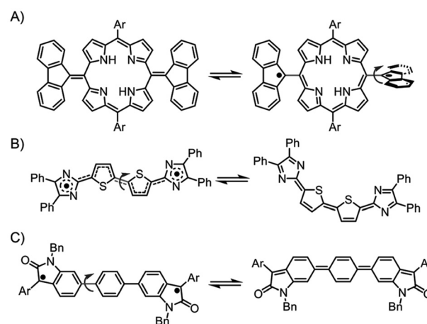
Fig. 1 An example of a structural change in a diradical form (A). Thermal cis – trans isomerization of Chichibabin's hydrocarbon analogues (B and C).
