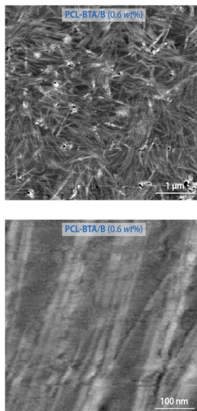
Figure 6. Intermittent-contact AFM phase images of PCL-BTA/B (0.6 wt%) recorded at 70 °C at different magnifications. See Supplementary Figure S13.
