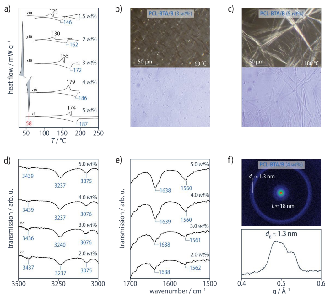
Figure 4. a) DSC heating and cooling scans (10 °C/min, exothermal transitions up) from the PCL-BTA/B blends for B concentrations \geq 1.5 wt%. For clarity, the PCL melting and crystallization transitions at T_m = 58 °C and T_c = 35 °C, respectively, are only shown for one composition. b, c) Cross-polarized (top) and bright-field (bottom) optical micrographs of PCL-BTA/B recorded at T < T_{agg} during cooling at 10 °C/min from the melt state. PCL-BTA/B blends containing \geq 1.5 wt% B show microfibrous precipitates (see also Supplementary Figure S12). d) The N–H stretching band, and e) the C=O stretching band and the combined N–H bending/C–N stretching band from ATR FTIR spectra of PCL-BTA/B recorded at 25 °C. The sharp absorption visible in all the spectra at 3435–3445 cm -1 is assigned to water absorption by the PCL. 92 f) The corresponding structures show Bragg reflections in the neighborhood of q \approx 0.24 Å -1 ( d_B \approx 1.3 nm) in XRD patterns obtained at room temperature.
