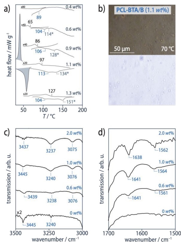
Figure 5. a) DSC heating and cooling scans (10 °C/min, exothermal transitions up) from PCL-BTA/B blends. For clarity, the PCL melting and crystallization transitions at T_m = 58 °C and T_c = 35 °C, respectively, are only shown for one composition. b) Cross-polarized (top) and bright-field (bottom) optical micrographs of PCL-BTA/B recorded at T < T_{agg} during cooling at 10 °C/min from the melt state. PCL-BTA/B blends at w_B \leq 1.1 wt% remain optically homogeneous (see also Supplementary Figure S12), but ATR FTIR spectra of PCL-BTA/B recorded at 25 °C contain c) the N-H stretching band and d) the C=O stretching band and the combined N-H bending/C-N stretching band indicative of BTA aggregates at all B concentrations investigated. The sharp absorption visible in all the spectra at 3435–3445 cm -1 is assigned to water absorption by the PCL. 92
