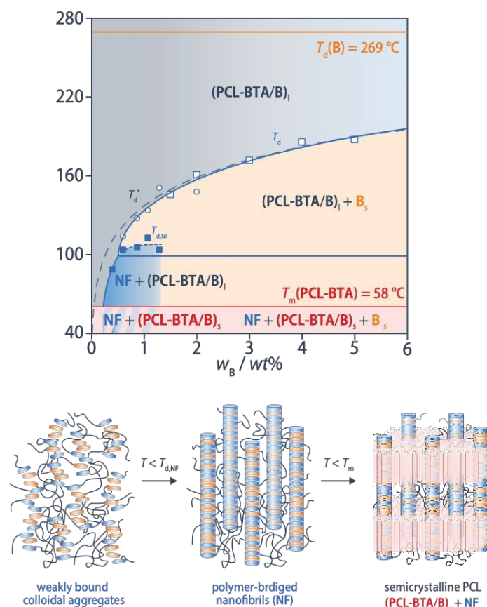
Figure 8. Phase diagram of PCL-BTA/B blends constructed from T_d^* (open circles), T_{d,NF} (filled squares) and T_d (open squares) obtained from DSC heating scans of PCL-BTA/B blends. (PCL-BTA/B) l – homogeneous melt; NF – nanofibrils; B s – bulk B precipitates; (PCL-BTA/B) s – solid solution. The grey dashed line is the fit of the Flory-Huggins model to T_d for PCL/B (see Figure 2).
