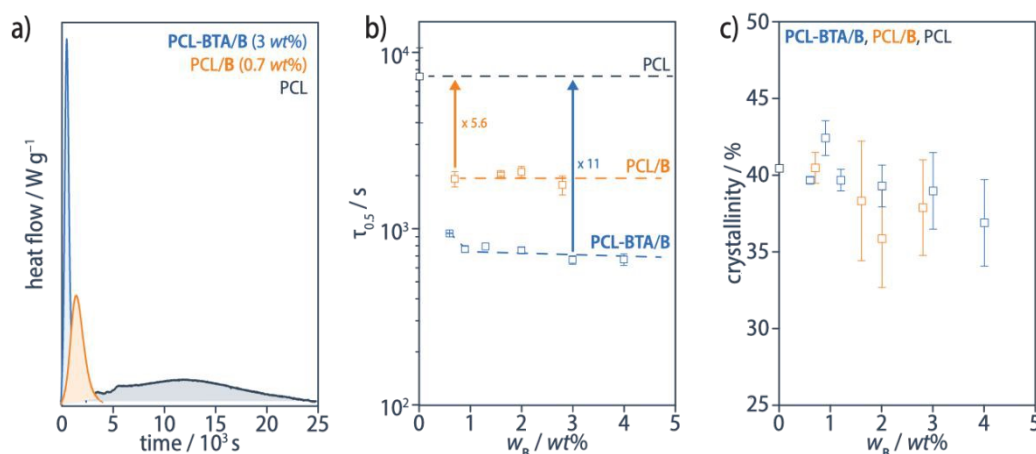
Figure 11. a) Examples of isothermal DSC traces for PCL-BTA/B (blue), PCL/ B (orange) and pristine PCL (grey) at 48 °C after cooling from 200 °C at 10 °C/min to 70 °C, followed by rapid cooling to 48 °C, from which b) the crystallization half times \tau_{1/2} have been determined. \tau_{1/2} is decreased by a factor of up to 5.6 in PCL/ B (orange), and up to 11 in blends of PCL-BTA/B (blue) compared with pristine PCL (grey). The dashed curves serve as guide to the eye. c) The degree of crystallinity of the PCL matrix as determined by integrating the PCL melting peak in heating scans at 10 °C/min recorded immediately after the isothermal step, assuming the melting enthalpy of an ideal PCL crystal to be 139.5 J/g. 95
