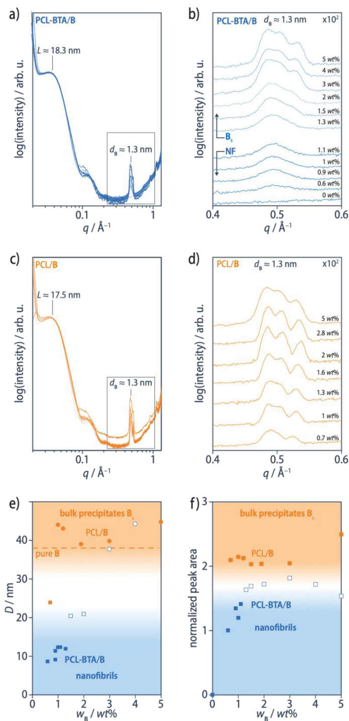
Figure 7. a) 1D SAXS diffractograms of PCL-BTA/B blends, measured on flat specimens obtained by cooling from the melt at -10\text{ }^{\circ}\text{C}/\text{min} , normalized with respect to the intense low q Bragg peaks corresponding to the lamellar long period, L , of the PCL matrix at about 17–18 nm. b) Enlargement of the Bragg reflections in the neighborhood of q \approx 0.24\text{ }\text{\AA}^{-1} ( d_B \approx 1.3\text{ nm} ). c,d) Corresponding 1D SAXS diffractograms of PCL/B blends. e) Total area of the Bragg peaks in the neighborhood of q \approx 0.24\text{ }\text{\AA}^{-1} divided by the B concentration and plotted against the B concentration, and f) the crystallite size, D , estimated from \beta for the Bragg reflections at d_B \approx 1.3\text{ nm} using the Scherrer equation (2), in both the PCL/B (orange symbols) and PCL-BTA/B blends (blue symbols – filled symbols for the NF regime, open symbols for the regime in which bulk precipitates become visible in OM); the dashed line corresponds to D estimated from \beta for bulk B , for which extrinsic factors such as instrumental broadening are assumed be significant.
