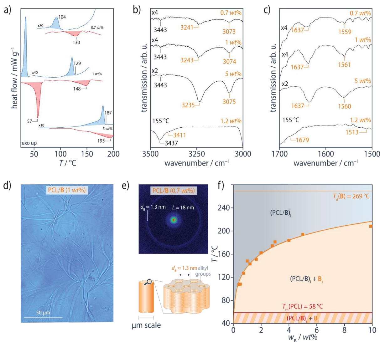
Figure 2. a) DSC heating (red) and cooling (blue) scans of PCL/ B at 10 °C/min for different B concentrations. For clarity, the PCL melting and crystallization transitions at T_m = 58 \text{ °C} and T_c = 35 \text{ °C} , respectively, are only shown for 1 wt% B . b) ATR FTIR spectra at room temperature show the N–H stretching band at 3235–3243 cm -1 , c) the C=O stretching band at 1637 cm -1 , and the combined N–H bending/C–N stretching band at 1559–1561 cm -1 , characteristic of strongly hydrogen-bonded amides in extended aggregates of B , all of which shift to positions corresponding to free amides 90 in FTIR transmission spectra recorded at 155 °C from a film of PCL/ B (1.2 wt%) on KBr. d) Optical micrographs show micrometer-sized fibrous precipitates of B , formed by lateral aggregation of the individual stacks, giving e) Bragg reflections in the neighborhood of q \approx 0.24 \text{ \AA}^{-1} ( d_B \approx 1.3 \text{ nm} ) in XRD patterns obtained at room temperature. f) Phase diagram for the PCL/ B reference blends, constructed from T_d determined from DSC heating scans. The PCL/ B blends form an optically transparent, homogeneous melt, (PCL/ B ) i , at sufficiently high temperatures.
