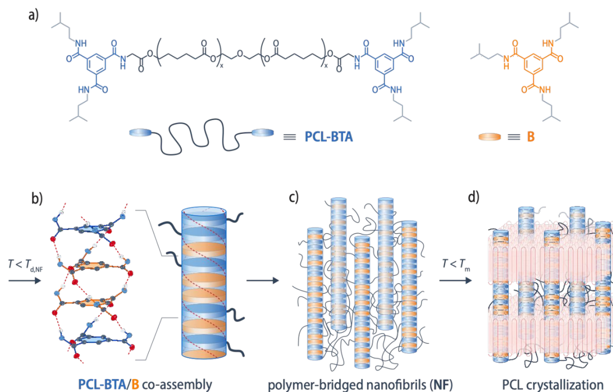
Figure 1. a) Chemical structure of end-modified PCL-BTA , and the matching additive B . On cooling, the end groups of PCL-BTA/B co-assemble with B by three-fold hydrogen bonding into b) polymer-tethered nanofibrils comprising one-dimensional stacks of BTA end groups and additive molecules. c) In the bulk materials, the nanofibrils are bridged by the polymer segments and d) coexist with crystalline PCL lamella upon cooling to T < T_m . For clarity the alkyl side chains of B have been omitted in b–d).
