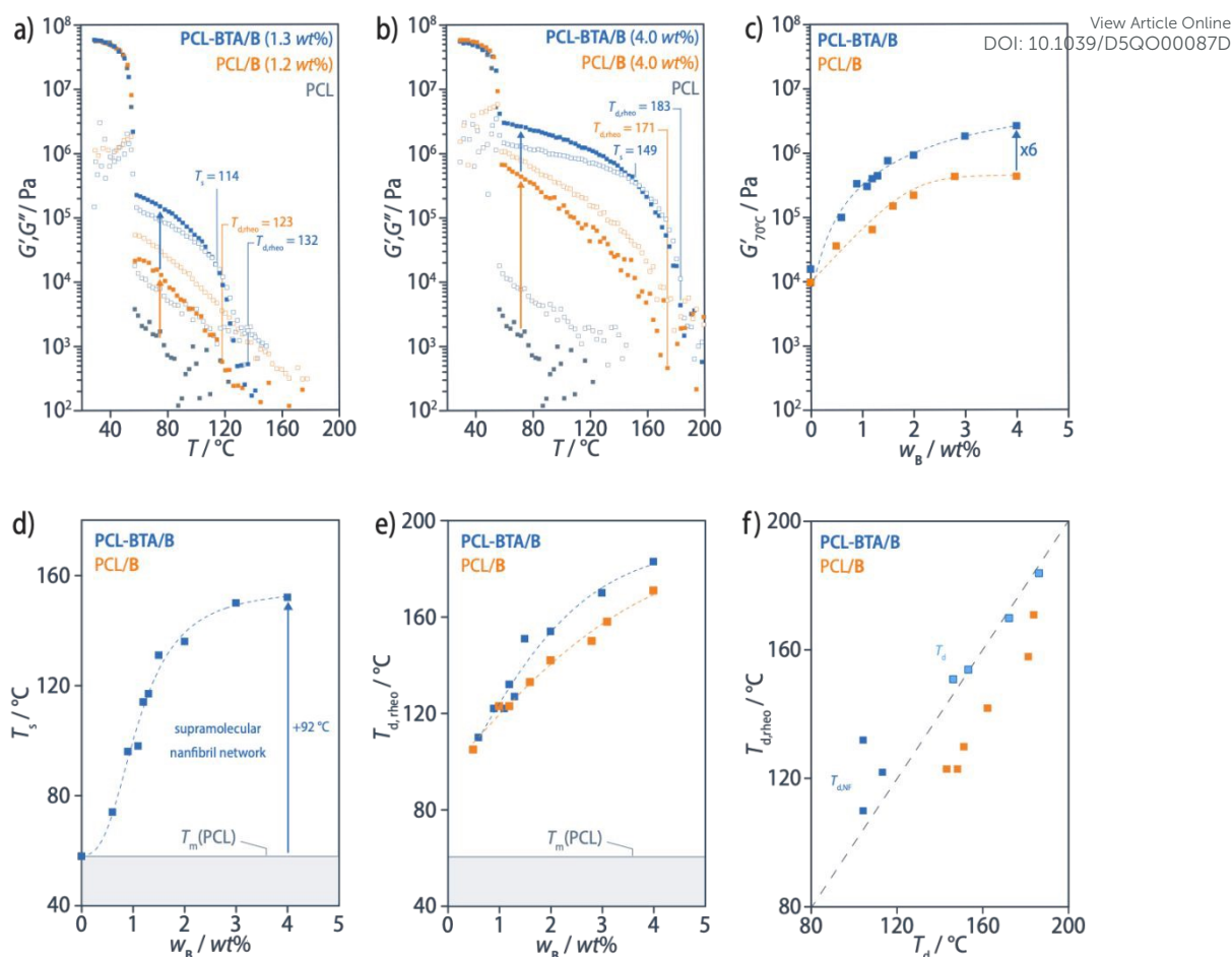
Figure 9. a,b ) Representative plots of the storage ( G' , filled squares) and loss ( G'' , open squares) moduli obtained from oscillatory shear rheometry heating scans for the PCL-BTA/B (blue) and PCL/B blends (orange) at a frequency of 1 rad/s and a scanning rate of 10 °C/min. Data for other B contents are shown in Supplementary Figure S15. c ) G' at 70 °C increases systematically with w_B as do d ) the softening temperature, T_s , above which G' > G'' (not observed for PCL/B ) and e ) T_{d,rheo} . f ) In PCL-BTA/B , T_{d,rheo} corresponds to either T_{d,NF} , for w_B \leq 1.1 wt%, or T_d for w_B \geq 1.5 wt% determined from DSC heating scans, but is slightly lower in PCL/B particularly at low B concentrations. Similar trends are also observed for G' at 70 °C, T_s , and T_{d,rheo} when plotted against the total concentration of BTA moieties, including the end groups, w_B + w_{BTA} (see Supplementary Figure S16). The dashed curves in all panels serve as guide to the eye.
