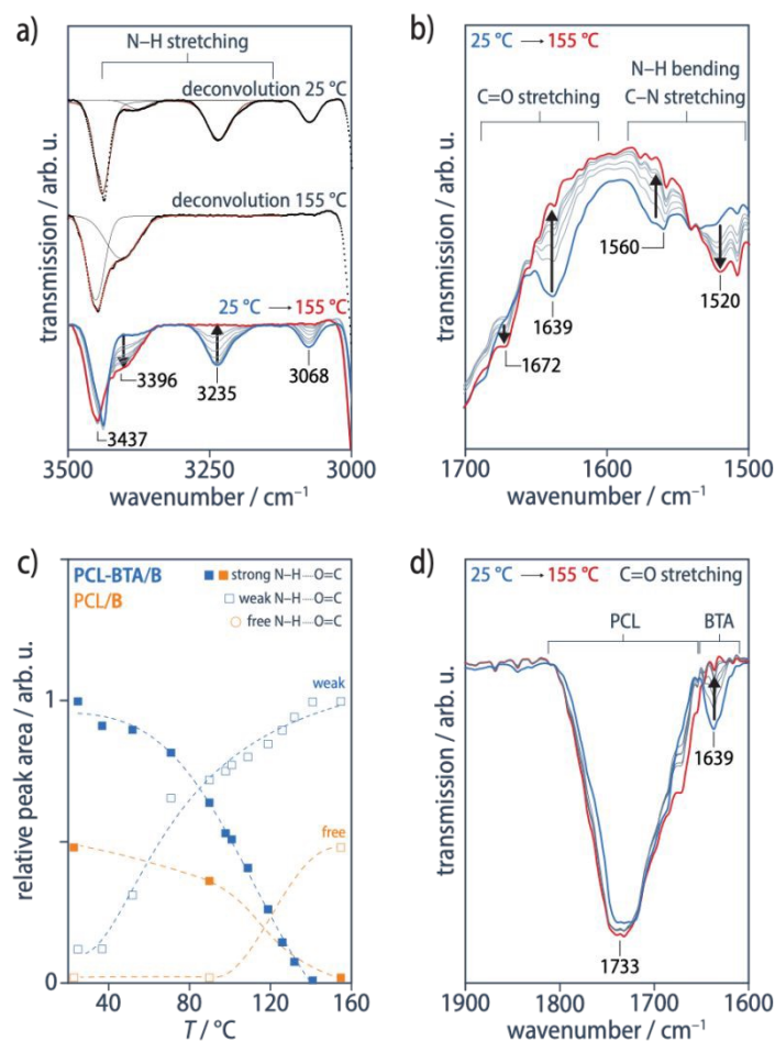
Figure 3. FTIR transmission spectra of a PCL-BTA/B (1 wt%) film on KBr, recorded at 25, 79, 101, 119, 126, 132, and 155 °C, respectively, showing a ) the N-H stretching band, with examples of the deconvolution of the spectrum at 25 and 155 °C, and b ) the C=O stretching band and the combined N-H bending/C-N stretching band. The ensemble of the deconvoluted spectra are shown in Supplementary Figure S11. The sharp absorption visible in all the spectra at 3435–3445 \text{cm}^{-1} is assigned to water absorption by the PCL. 92 c ) The area of the N-H stretching peak obtained from the deconvoluted spectra of PCL-BTA/B (1 wt%) (blue) and PCL/B (1.2 wt%) (orange), normalized with respect to the area of the PCL C–H 2 stretching peak (not shown). The dashed curves serve as guide to the eye. d ) The C=O stretching band of the PCL backbone does not change with temperature.
