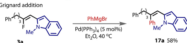
Fig. 3 Mechanistic control reactions for \beta -fluorovinyl indole synthesis and preliminary derivatisation studies.
