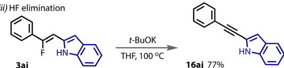
Fig. 3 Mechanistic control reactions for \beta -fluorovinyl indole synthesis and preliminary derivatisation studies.
