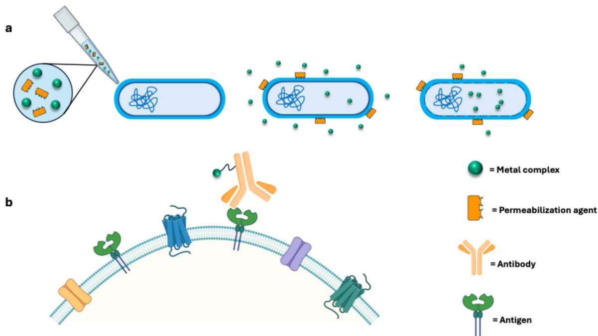
Fig. 2 Graphical representation of the two most exploited combination therapy approaches. (a) Combined action of a permeabilizing agent (orange) and a metal complex (green sphere). The presence of the permeabilizing agent facilitates the disruption of the bacterial membrane wall (represented as a dashed blue line) increasing the effective presence of the metal compound inside the bacteria (b) metal complexes can be covalently linked to antibodies specific residues. The formed bioconjugate can specifically interact with the corresponding antigen on the bacterial wall surface.
