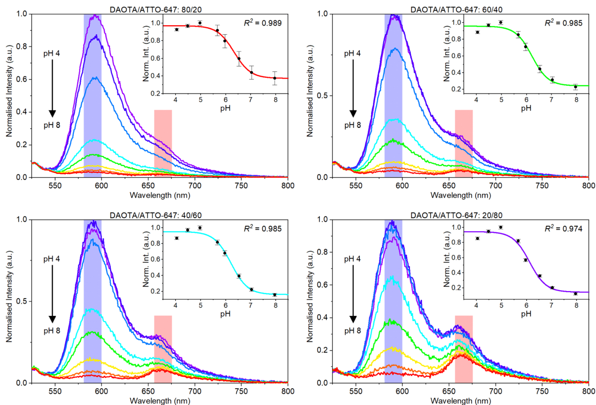
Fig. 3 Fluorescence emission spectra of pH titrations ( \lambda_{\text{Ex}} = 510 \text{ nm} ), showing the effect of changing the DAOTA/ATTO-647 loading ratio on emission spectra and response curves (insets). The response curves were calculated as the ratio between the summed response signal (blue area) and the summed reference signal (red area), emulating the emission bands that were used during plate reader measurements. Error bars are calculated from the instrumental response error.
