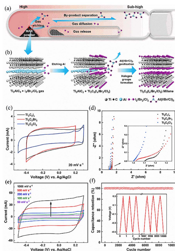
Fig. 5 (a and b) Mechanism of gas-phase selective dry etching. (c) CV curves of \text{Ti}_3\text{C}_2\text{I}_x , \text{Ti}_3\text{C}_2\text{Br}_x , and \text{Ti}_3\text{C}_2\text{Cl}_x at a scan rate of 20 \text{ mV s}^{-1} . (d) EIS curves of \text{Ti}_3\text{C}_2\text{I}_x , \text{Ti}_3\text{C}_2\text{Br}_x , and \text{Ti}_3\text{C}_2\text{Cl}_x ; (e) CV curves of \text{Ti}_3\text{C}_2\text{I}_x , \text{Ti}_3\text{C}_2\text{Br}_x , and \text{Ti}_3\text{C}_2\text{Cl}_x at 50, 100, 200, 500 and 1000 \text{ mV s}^{-1} scan rates. (f) cycling stability at a current density of 5 \text{ mA cm}^{-2} . Reproduced from ref. 81 with permission from [Elsevier], copyright [2024].
