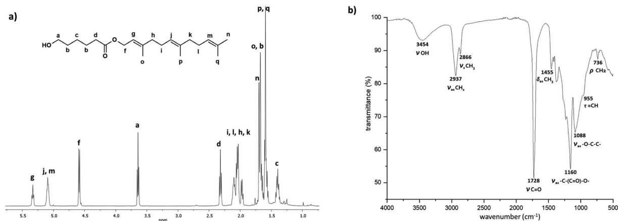
Fig. 3 Spectra of a monomer C_{15}F-CL_1 (monodisperse oligomeric specie, Table 2) isolated by FCC from C_{15}F-PCL (Table 1). (a) ^1H NMR (500 MHz) in CDCl_3 , and (b) FTIR.
