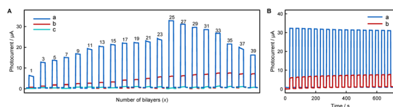
Fig. 3 (A) Photocurrent responses of (MV/AuNPs) x /FTO (a), (NR/AuNPs) x /FTO (b), and (AuNPs) x /FTO (c) electrodes ( x = 1, 3, 5, \dots, 39 ). (B) Stability of (MV/AuNPs) 25 /FTO (a) and (NR/AuNPs) 33 /FTO (b) electrodes. The photocurrents were measured in 0.1 M PBS (pH 7.4) containing 0.1 M AA at 0 V vs. SCE.
