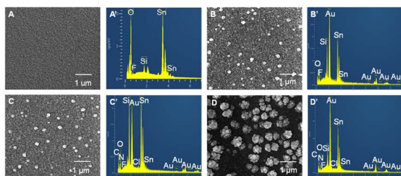
Fig. 2 SEM and EDX images of FTO (A and A'), AuNPs/FTO (B and B'), MV/AuNPs/FTO (C and C'), and (MV/AuNPs) 25 /FTO (D and D'). The large white particles in the SEM images are AuNPs.
