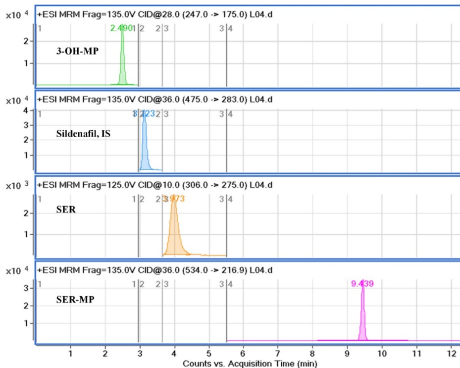
Fig. 2 Representative MRM chromatograms of standard sertraline solution, 25 \text{ ng mL}^{-1} at 3.97 min; SER-MP, 0.25 \text{ ng mL}^{-1} at 9.43 min; 3-OHMP, 25 \text{ ng mL}^{-1} at 2.49 min; and internal standard, 20 \text{ ng mL}^{-1} at 3.22 min.
