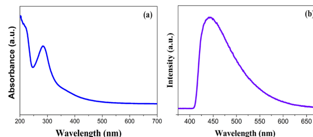
Fig. 1 (a) UV absorption and (b) PL spectrum of ACDs.
