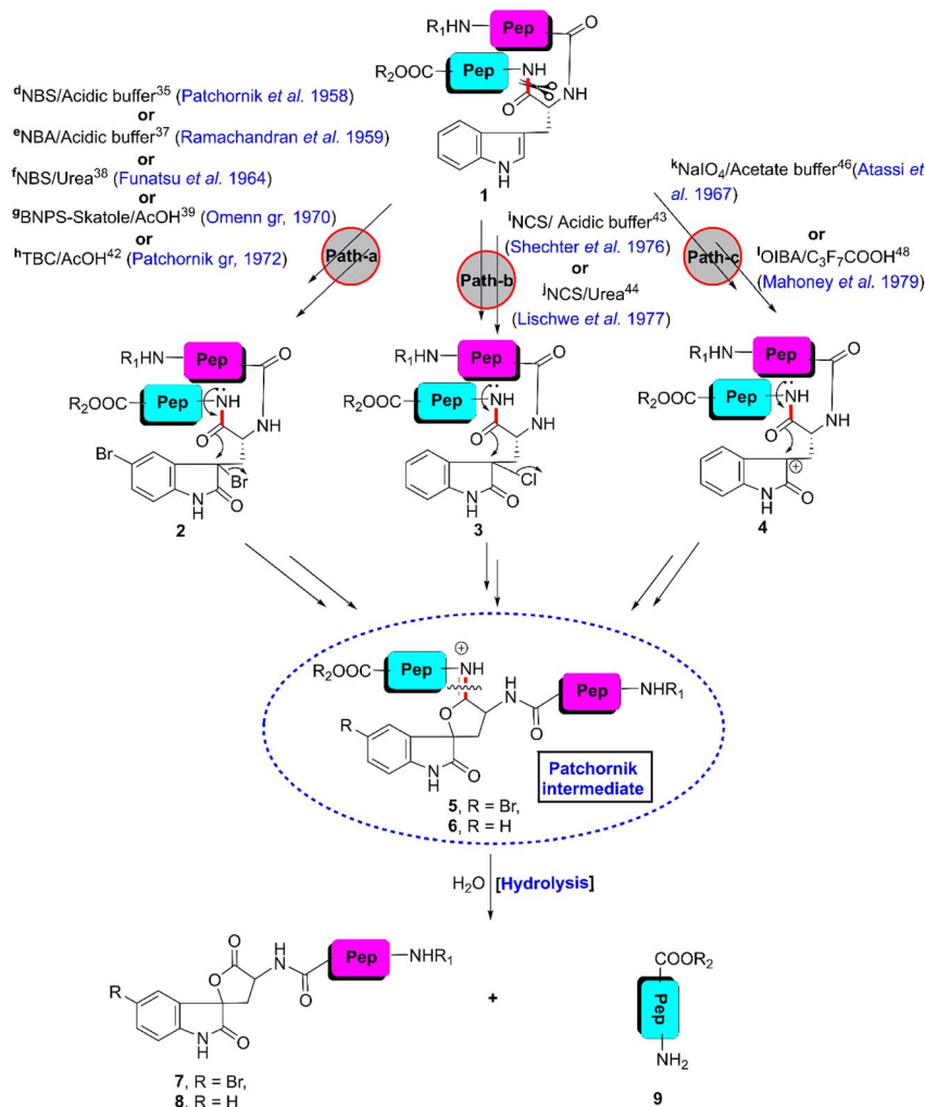
Fig. 2 W-selective scissoring of peptides/proteins through chemical oxidation. [Reaction conditions: ^d\text{NBS} , aqueous acetate buffer (pH 4), RT, <1 min, 5–8%; ^e\text{NBA} , acidic buffer (pH 4), RT, 15–20 min, 20–40%; ^f\text{NBS} , 8 (M) aqueous urea, RT, 200 min, yield not reported; ^g\text{BNPS-skatole/AcOH} , RT, 20–30 min, 15%; ^h\text{TBC/AcOH} (pH 3), RT, 5–15 min, 50%; ^i\text{NCS/50–80\% acetic acid} (pH 4–5), RT, 30 min, 35–40%; ^j\text{NCS} , 4.68 (M) urea, 27.5% acetic acid, RT, 30 min, 50%; ^k\text{NaIO}_4 , acetate buffer (pH 5), 0 °C, followed by acidic hydrolysis at RT, 92–94% at W-7 & 17–22% at W-14 of SWM; ^l\text{OIBA} , 80% acetic acid, RT, 30 min, 70–100%].
