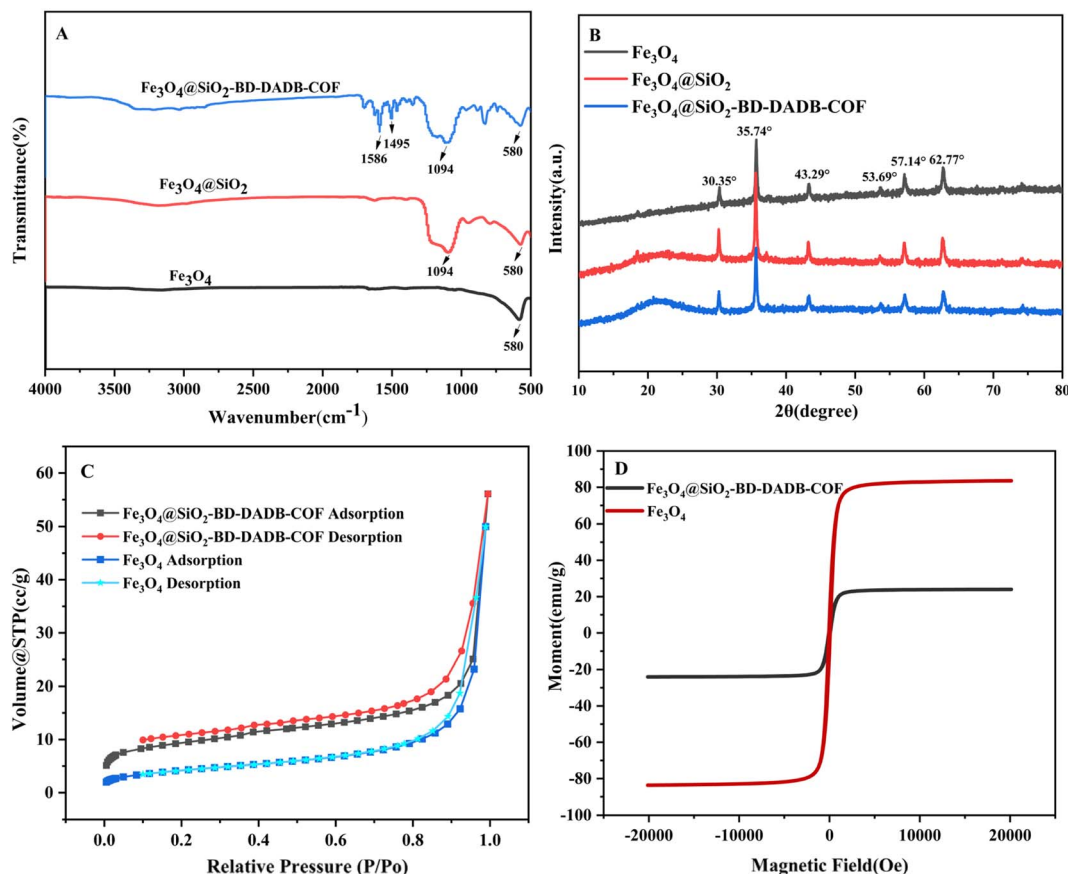
Fig. 3 (A) FT-IR spectra of \text{Fe}_3\text{O}_4 , \text{Fe}_3\text{O}_4@\text{SiO}_2 and \text{Fe}_3\text{O}_4@\text{SiO}_2\text{-BD-DADB-COF} ; (B) XRD patterns of \text{Fe}_3\text{O}_4 , \text{Fe}_3\text{O}_4@\text{SiO}_2 and \text{Fe}_3\text{O}_4@\text{SiO}_2\text{-BD-DADB-COF} ; (C) \text{N}_2 adsorption-desorption isotherms of \text{Fe}_3\text{O}_4 and \text{Fe}_3\text{O}_4@\text{SiO}_2\text{-BD-DADB-COF} ; (D) VSM curves of \text{Fe}_3\text{O}_4 and \text{Fe}_3\text{O}_4@\text{SiO}_2\text{-BD-DADB-COF} .
