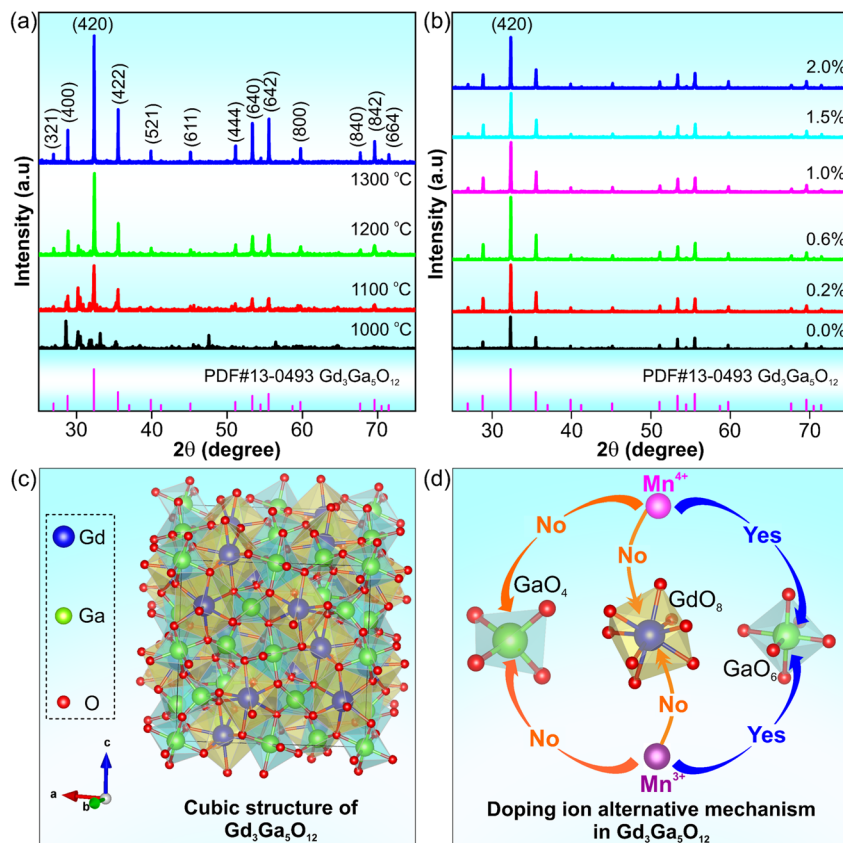
Fig. 1 XRD patterns of (a) Gd 3 Ga 5 O 12 :0.2% Mn phosphors annealed at various temperatures and (b) Gd 3 Ga 5 O 12 :x% Mn ( x = 0.0–2.0 ) phosphors annealed at 1300 °C (c) cubic structure of the Gd 3 Ga 5 O 12 lattice modeled using VESTA software and (d) preferred substitution of Mn 3+ and Mn 4+ ions for Ga 3+ ions [GaO 6 ] sites in the Gd 3 Ga 5 O 12 lattice.
