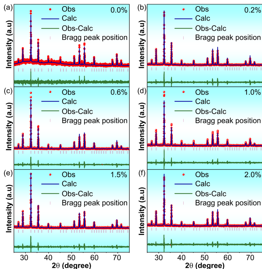
Fig. 2 Rietveld refinement for the \text{Gd}_3\text{Ga}_5\text{O}_{12}:x\%\text{Mn} ( x = 0.0\text{--}2.0 ) phosphors annealed at 1300\text{ }^\circ\text{C} for 5 hours in air.
