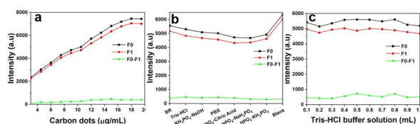
Fig. 6 (a) The optimal WCS-CDs concentration in the detection system; (b) the optimal type of buffer solution in the detection system; (c) the optimal buffer solution content in the detection system.
