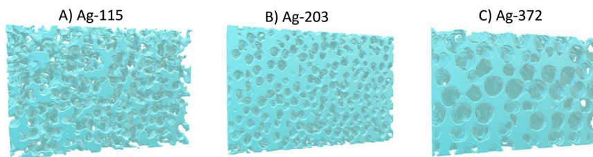
Fig. 7 3D reconstruction based on the FIB-SEM slice-and-view results from the samples A) Ag-115; B) Ag-203; and C) Ag-372.
