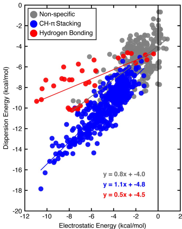
Fig. 3 Comparison of SAPTO dispersion and electrostatic energies for the three categories of interactions: CH- \pi stacking interactions (blue), hydrogen bonding interactions (red), and non-specific interactions (gray), of the full dataset. Best-fit lines for the CH- \pi stacking interactions (blue), hydrogen bonding interactions (red), and other close contacts (gray) are shown. All energies are reported in kcal mol -1 . SAPTO energies were evaluated using the aug-cc-pVDZ basis set.
