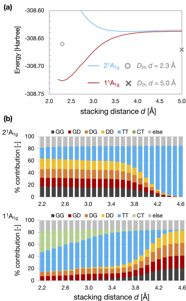
Fig. 4 Energies of 1^1A_g and 2^1A_g states of D_{4h} -dimer model as a function of stacking distance d and weight of electron configurations (b). The cross and circle in Fig. 4(a) represent the total energy calculated for the D_{2h} -dimer model at d = 5.0 Å and 2.3 Å.
