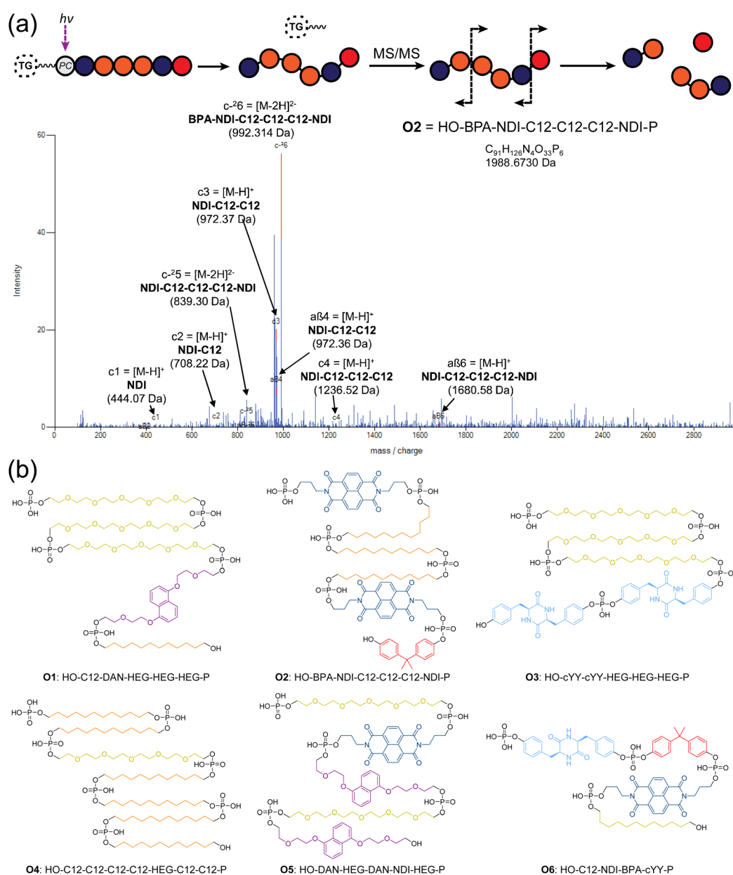
Fig. 4 (a) RoboOligo analysis of O2 . Other major peaks are indexed on alternative fragments (see ESI Section 5.2†). (b) Sequences of top binding phosphoestamers. Sequences are given by analogy with nucleic acid conventions (5' to 3') meaning that the first monomer listed is the last one added during chemical synthesis. This is evident from the location of the terminal phosphate which exists in the MS/MS spectra as a result of the photocleavage reaction, leading to the HO- and -P (phosphate) termini.
